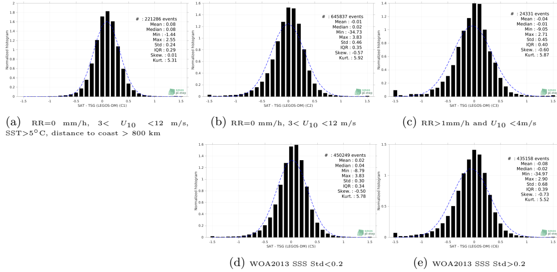
Figure 13: Normalized histogram of \Delta SSS (SMAP SSS L3 v5.0 - 8-Day running (JPL) - TSG (LEGOS-DM)) for 5 different subdatasets corresponding to: RR=0 mm/h, 3 < U_{10} < 12 m/s, SST >5^{\circ} C, distance to coast > 800 km (a), RR=0 mm/h, 3 < U_{10} < 12 m/s (b), RR >1 mm/h and U_{10} < 4 m/s (c), WOA2013 SSS Std <0.2 (d), WOA2013 SSS Std >0.2 (e).
