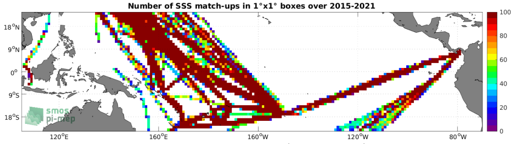
Figure 4: Number of SSS match-ups between TSG (LEGOS-DM) SSS and the SMAP SSS L3 v5.0 - 8-Day running (JPL) SSS product for the Tropical Pacific Ocean Pi-MEP region over 1^\circ \times 1^\circ boxes and for the full satellite product period.
