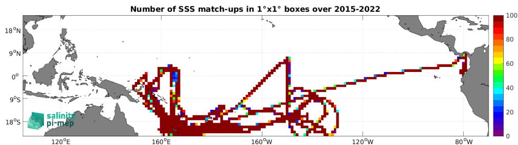
Figure 5: Number of SSS match-ups between TSG (GOSUD-Research-vessel) SSS and the SMAP SSS L3 v5.0 - 8-Day running (JPL) SSS product for the Tropical Pacific Ocean Pi-MEP region over 1^\circ \times 1^\circ boxes and for the full satellite product period.
