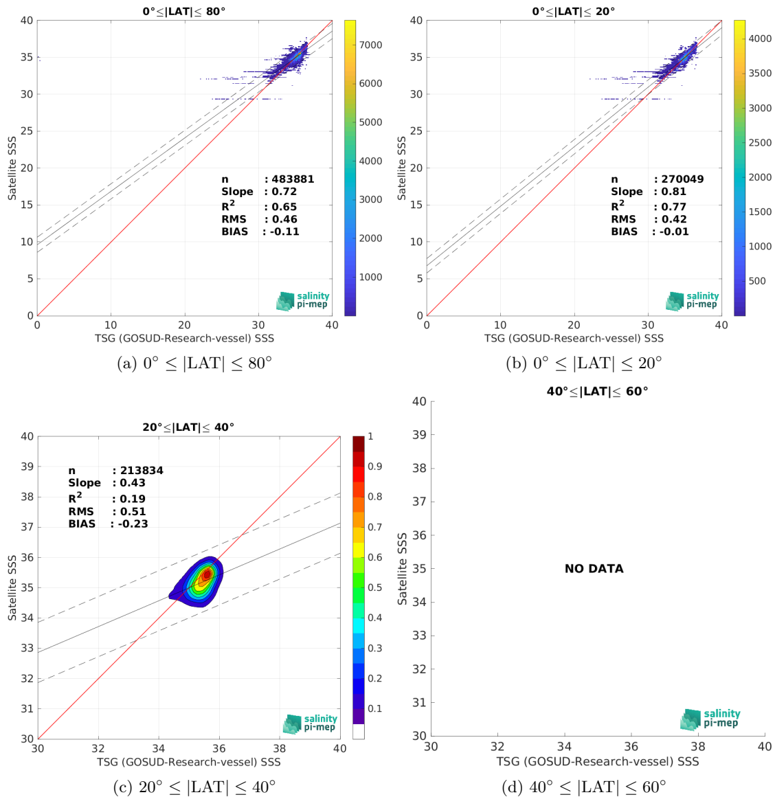
Figure 10: Contour maps of the concentration of SMAP SSS L3 v5.0 - 8-Day running (JPL) SSS (y-axis) versus TSG (GOSUD-Research-vessel) SSS (x-axis) at match-up pairs for different latitude bands. For each plot, the red line shows x=y . The black thin and dashed lines indicate a linear fit through the data cloud and the \pm 95\% confidence levels, respectively. The number of match-up pairs n , the slope and R^2 coefficient of the linear fit, the root mean square (RMS) and the mean bias between satellite and in situ data are indicated for each latitude band in each plot.
