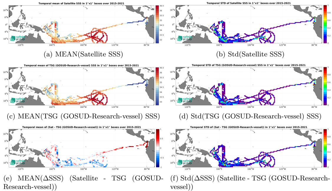
Figure 7: Temporal mean (left) and Std (right) of SSS from SMAP SSS L3 v5.0 - 8-Day running (JPL) (top), TSG (GOSUD-Research-vessel) (middle), and of \Delta SSS (Satellite - TSG (GOSUD-Research-vessel)). Only match-up pairs are used to generate these maps.
