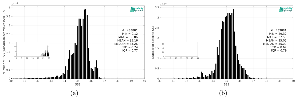
Figure 3: Histograms of SSS from TSG (GOSUD-Research-vessel) (a) and SMAP SSS L3 v5.0 - 8-Day running (JPL) (b) considering all match-up pairs per bins of 0.1 over the Tropical Pacific Ocean Pi-MEP region and for the full satellite product period.
