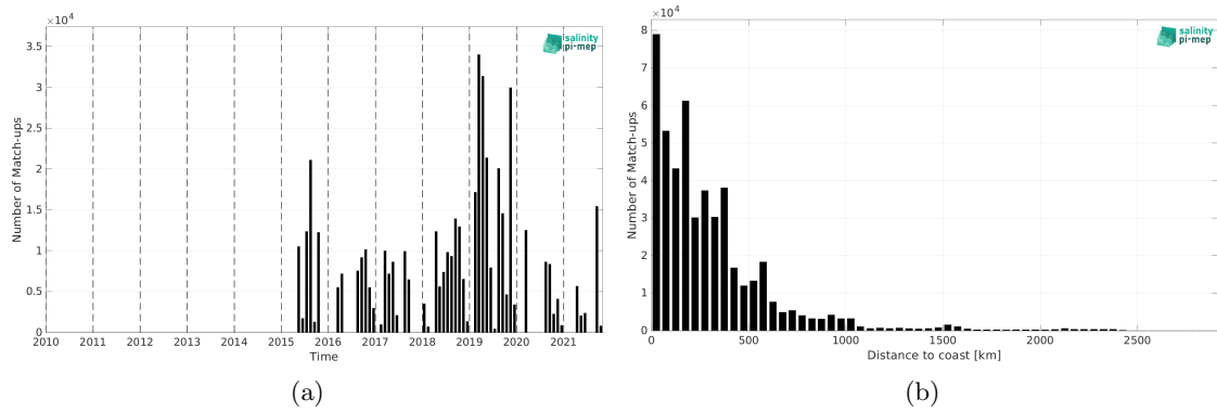
Figure 2: Number of match-ups between TSG (GOSUD-Research-vessel) and SMAP SSS L3 v5.0 - 8-Day running (JPL) SSS as a function of time (a) and as function of the distance to coast (b) over the Tropical Pacific Ocean Pi-MEP region and for the full satellite product period.
