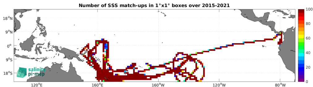
Figure 5: Number of SSS match-ups between TSG (GOSUD-Research-vessel) SSS and the SMAP SSS L3 v5.0 - 8-Day running (JPL) SSS product for the Tropical Pacific Ocean Pi-MEP region over 1°×1° boxes and for the full satellite product period.
