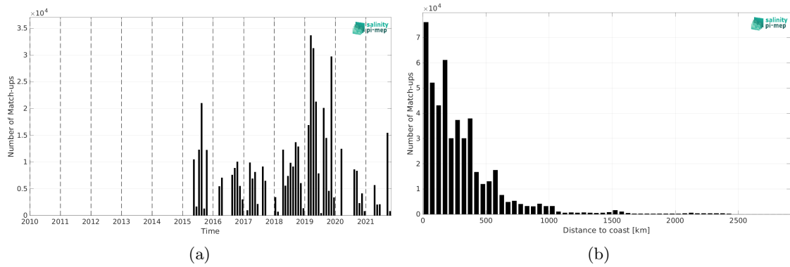
Figure 1: Number of match-ups between TSG (GOSUD-Research-vessel) and SMAP SSS L3 v5.0 - 8-Day running (JPL) SSS as a function of time (a) and as function of the distance to coast (b) over the Tropical Pacific Ocean Pi-MEP region and for the full satellite product period.
