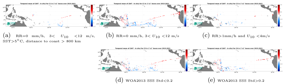
Figure 12: Temporal mean gridded over spatial boxes of size 1^\circ \times 1^\circ of \Delta SSS (SMAP SSS L3 v5.0 - 8-Day running (JPL) - TSG (GOSUD-Research-vessel)) for 5 different subdatasets corresponding to: RR=0 mm/h, 3 < U_{10} < 12 m/s, SST > 5^\circ\text{C} , distance to coast > 800 km (a), RR=0 mm/h, 3 < U_{10} < 12 m/s (b), RR > 1 mm/h and U_{10} < 4 m/s (c), WOA2013 SSS Std < 0.2 (d), WOA2013 SSS Std > 0.2 (e).
