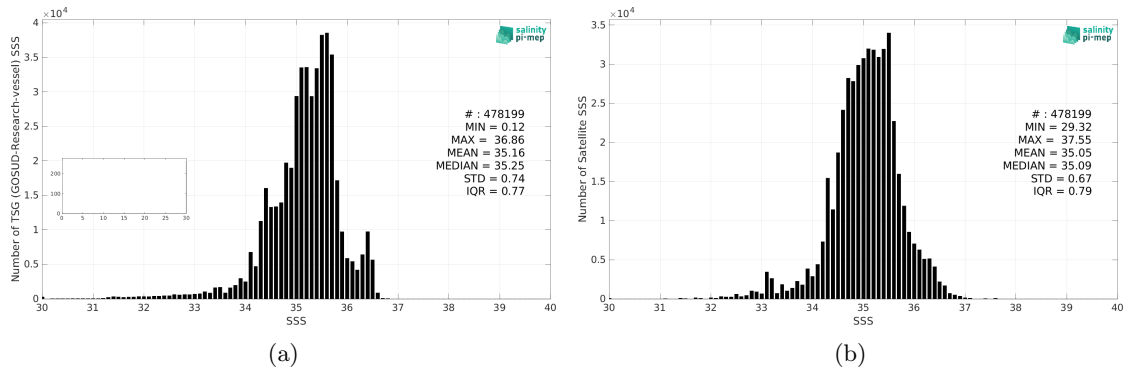
Figure 2: Histograms of SSS from TSG (GOSUD-Research-vessel) (a) and SMAP SSS L3 v5.0 - 8-Day running (JPL) (b) considering all match-up pairs per bins of 0.1 over the Tropical Pacific Ocean Pi-MEP region and for the full satellite product period.
