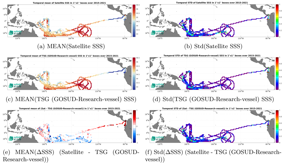
Figure 6: Temporal mean (left) and Std (right) of SSS from SMAP SSS L3 v5.0 - 8-Day running (JPL) (top), TSG (GOSUD-Research-vessel) (middle), and of \Delta SSS (Satellite - TSG (GOSUD-Research-vessel)). Only match-up pairs are used to generate these maps.
