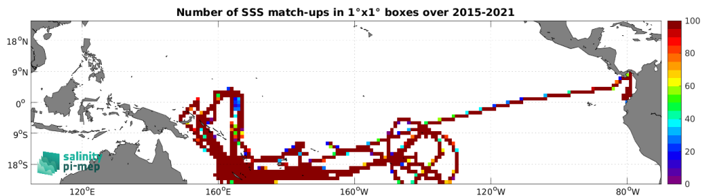
Figure 4: Number of SSS match-ups between TSG (GOSUD-Research-vessel) SSS and the SMAP SSS L3 v5.0 - 8-Day running (JPL) SSS product for the Tropical Pacific Ocean Pi-MEP region over 1^\circ \times 1^\circ boxes and for the full satellite product period.
