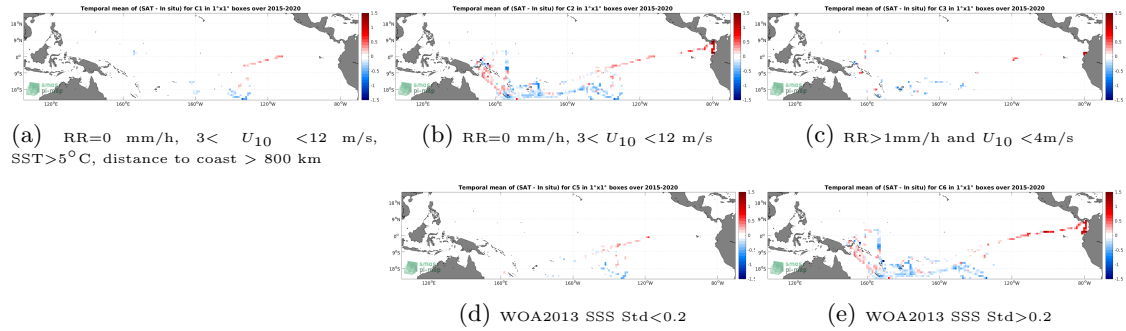
Figure 12: Temporal mean gridded over spatial boxes of size 1^{\circ}\times 1^{\circ} of \Delta SSS (SMAP SSS L3 v5.0 - 8-Day running (JPL) - TSG (GOSUD-Research-vessel)) for 5 different subdatasets corresponding to:RR=0 mm/h, 3 < U_{10} < 12 m/s, SST >5^{\circ}\text{C} , distance to coast > 800 km (a), RR=0 mm/h, 3 < U_{10} < 12 m/s (b), RR >1 mm/h and U_{10} < 4 m/s (c), WOA2013 SSS Std <0.2 (d), WOA2013 SSS Std >0.2 (e).
