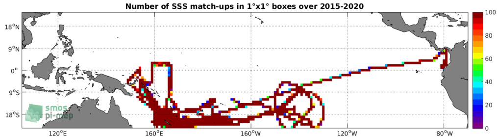
Figure 4: Number of SSS match-ups between TSG (GOSUD-Research-vessel) SSS and the SMAP SSS L3 v5.0 - 8-Day running (JPL) SSS product for the Tropical Pacific Ocean Pi-MEP region over 1^\circ \times 1^\circ boxes and for the full satellite product period.
