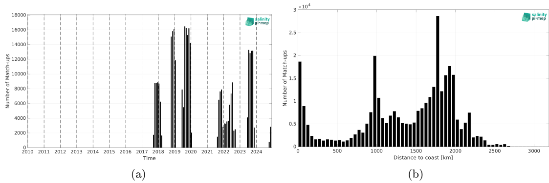
Figure 2: Number of match-ups between Sairdrone and SMAP SSS L3 v5.0 - 8-Day running (JPL) SSS as a function of time (a) and as function of the distance to coast (b) over the Tropical Pacific Ocean Pi-MEP region and for the full satellite product period.
