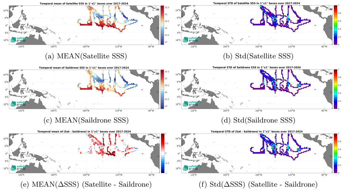
Figure 7: Temporal mean (left) and Std (right) of SSS from SMAP SSS L3 v5.0 - 8-Day running (JPL) (top), Saildrone (middle), and of \Delta SSS (Satellite - Saildrone). Only match-up pairs are used to generate these maps.
