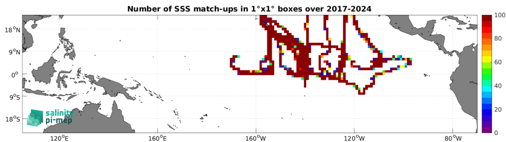
Figure 5: Number of SSS match-ups between Saildrone SSS and the SMAP SSS L3 v5.0 - 8-Day running (JPL) SSS product for the Tropical Pacific Ocean Pi-MEP region over 1^\circ \times 1^\circ boxes and for the full satellite product period.
