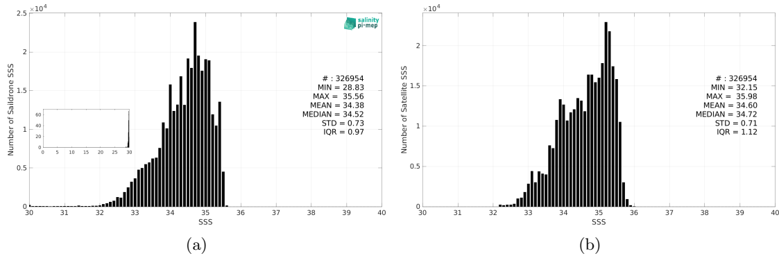
Figure 3: Histograms of SSS from Sairdrone (a) and SMAP SSS L3 v5.0 - 8-Day running (JPL) (b) considering all match-up pairs per bins of 0.1 over the Tropical Pacific Ocean Pi-MEP region and for the full satellite product period.
