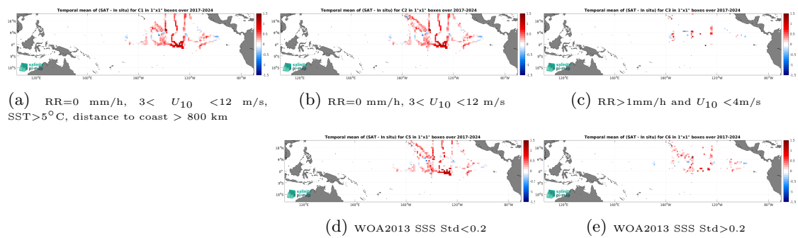
Figure 14: Temporal mean gridded over spatial boxes of size 1^\circ \times 1^\circ of \Delta\text{SSS} (SMAP SSS L3 v5.0 - 8-Day running (JPL) - Sairdrone) for 5 different subdatasets corresponding to:RR=0 mm/h, 3 < U_{10} < 12 m/s, SST > 5^\circ\text{C} , distance to coast > 800 km (a), RR=0 mm/h, 3 < U_{10} < 12 m/s (b), RR > 1 mm/h and U_{10} < 4 m/s (c), WOA2013 SSS Std < 0.2 (d), WOA2013 SSS Std > 0.2 (e).
