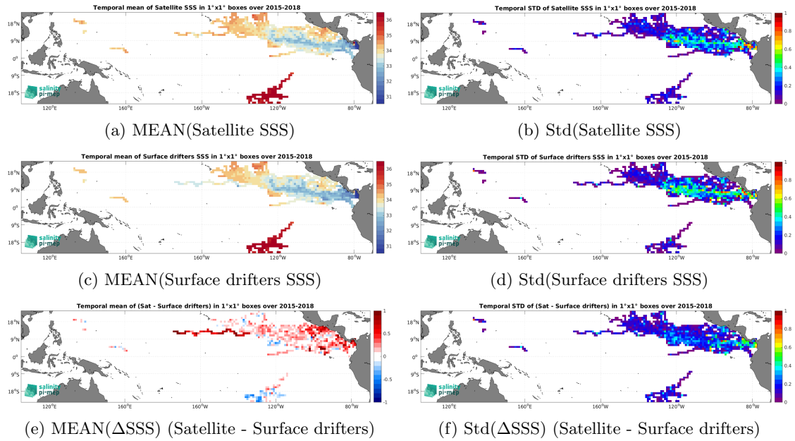
Figure 6: Temporal mean (left) and Std (right) of SSS from SMAP SSS L3 v5.0 - 8-Day running (JPL) (top), Surface drifters (middle), and of \Delta SSS (Satellite - Surface drifters). Only match-up pairs are used to generate these maps.
