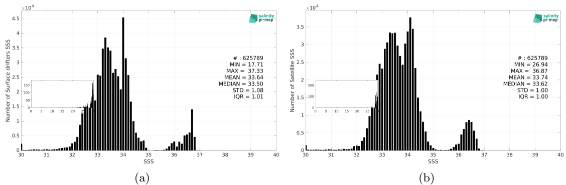
Figure 3: Histograms of SSS from Surface drifters (a) and SMAP SSS L3 v5.0 - 8-Day running (JPL) (b) considering all match-up pairs per bins of 0.1 over the Tropical Pacific Ocean Pi-MEP region and for the full satellite product period.
