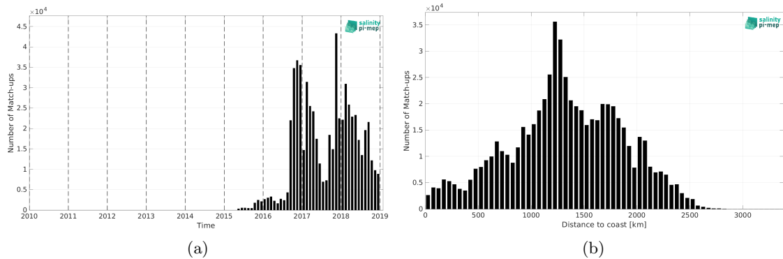
Figure 2: Number of match-ups between Surface drifters and SMAP SSS L3 v5.0 - 8-Day running (JPL) SSS as a function of time (a) and as function of the distance to coast (b) over the Tropical Pacific Ocean Pi-MEP region and for the full satellite product period.
