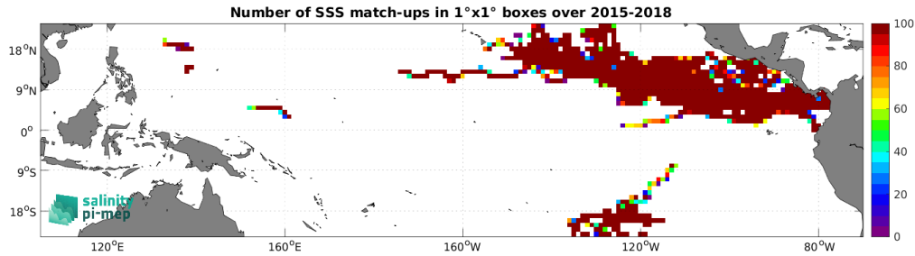
Figure 4: Number of SSS match-ups between Surface drifters SSS and the SMAP SSS L3 v5.0 - 8-Day running (JPL) SSS product for the Tropical Pacific Ocean Pi-MEP region over 1^\circ \times 1^\circ boxes and for the full satellite product period.
