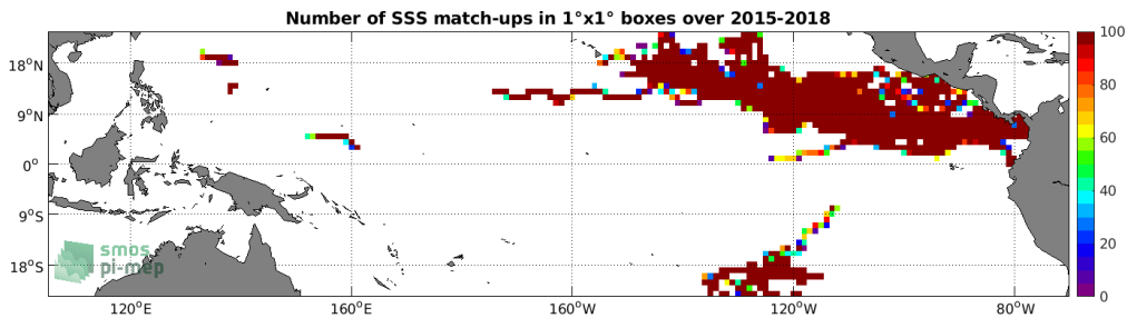
Figure 3: Number of SSS match-ups between Surface drifters SSS and the SMAP SSS L3 v5.0 - 8-Day running (JPL) SSS product for the Tropical Pacific Ocean Pi-MEP region over 1^\circ \times 1^\circ boxes and for the full satellite product period.
