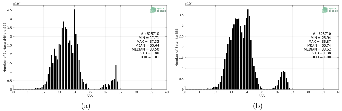
Figure 2: Histograms of SSS from Surface drifters (a) and SMAP SSS L3 v5.0 - 8-Day running (JPL) (b) considering all match-up pairs per bins of 0.1 over the Tropical Pacific Ocean Pi-MEP region and for the full satellite product period.
