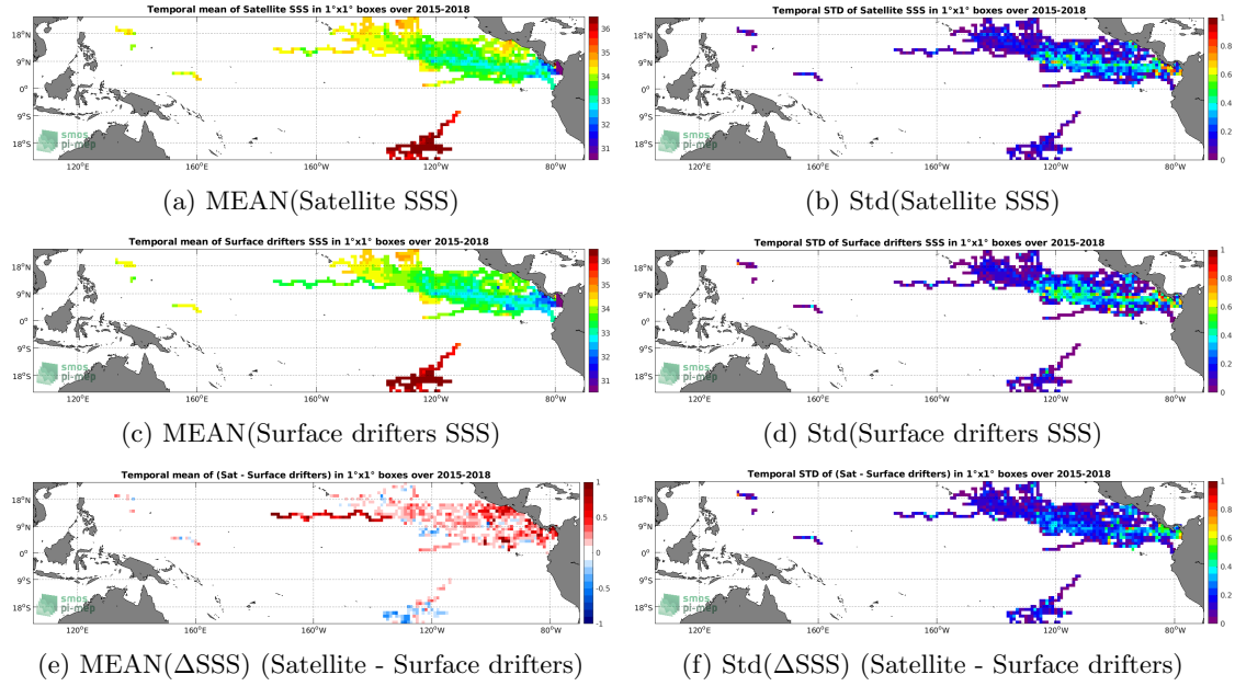
Figure 5: Temporal mean (left) and Std (right) of SSS from SMAP SSS L3 v5.0 - 8-Day running (JPL) (top), Surface drifters (middle), and of \Delta SSS (Satellite - Surface drifters). Only match-up pairs are used to generate these maps.
