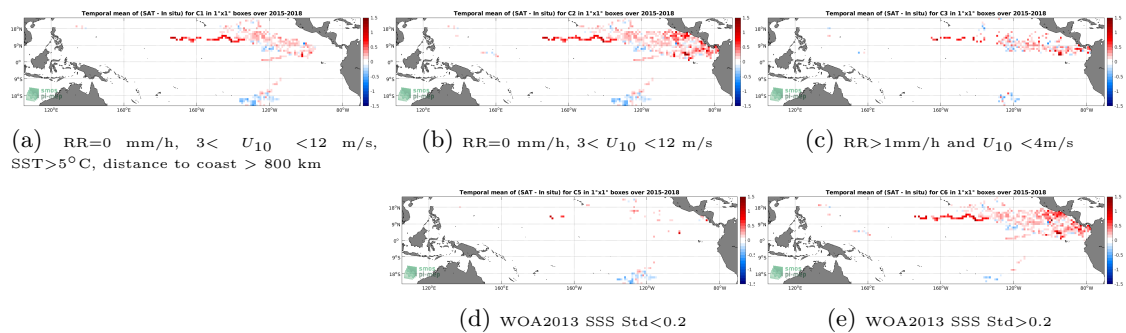
Figure 11: Temporal mean gridded over spatial boxes of size 1^\circ \times 1^\circ of \Delta SSS (SMAP SSS L3 v5.0 - 8-Day running (JPL) - Surface drifters) for 5 different subdatasets corresponding to:RR=0 mm/h, 3 < U_{10} < 12 m/s, SST >5^\circ\text{C} , distance to coast > 800 km (a), RR=0 mm/h, 3 < U_{10} < 12 m/s (b), RR >1 mm/h and U_{10} < 4 m/s (c), WOA2013 SSS Std <0.2 (d), WOA2013 SSS Std >0.2 (e).
