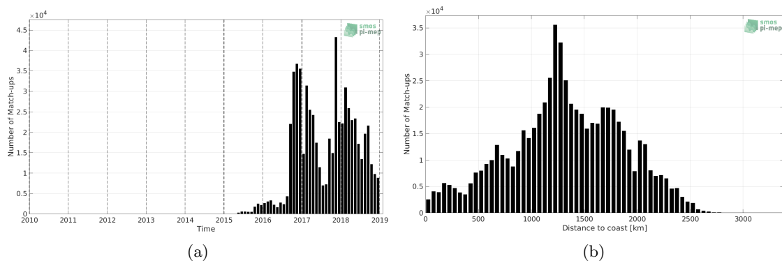
Figure 1: Number of match-ups between Surface drifters and SMAP SSS L3 v5.0 - 8-Day running (JPL) SSS as a function of time (a) and as function of the distance to coast (b) over the Tropical Pacific Ocean Pi-MEP region and for the full satellite product period.
