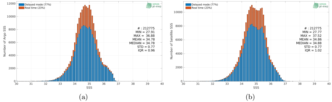
Figure 2: Histograms of SSS from Argo (a) and SMAP SSS L3 v5.0 - 8-Day running (JPL) (b) considering all match-up pairs per bins of 0.1 over the Tropical Pacific Ocean Pi-MEP region and for the full satellite product period.
