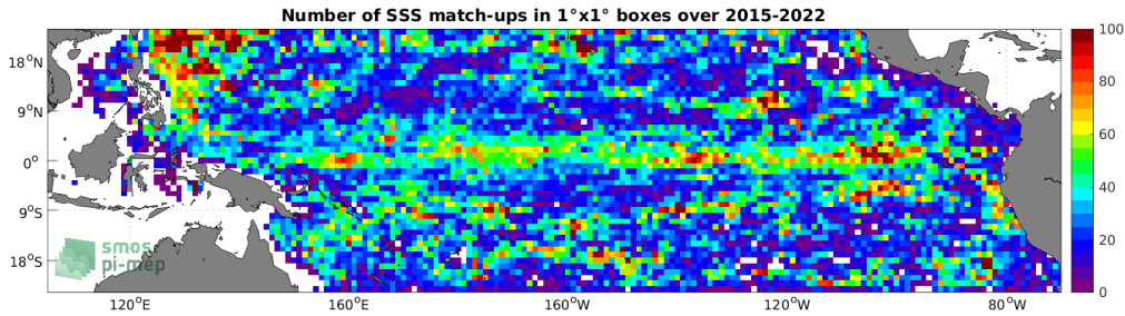
Figure 4: Number of SSS match-ups between Argo SSS and the SMAP SSS L3 v5.0 - 8-Day running (JPL) SSS product for the Tropical Pacific Ocean Pi-MEP region over 1^\circ \times 1^\circ boxes and for the full satellite product period.
