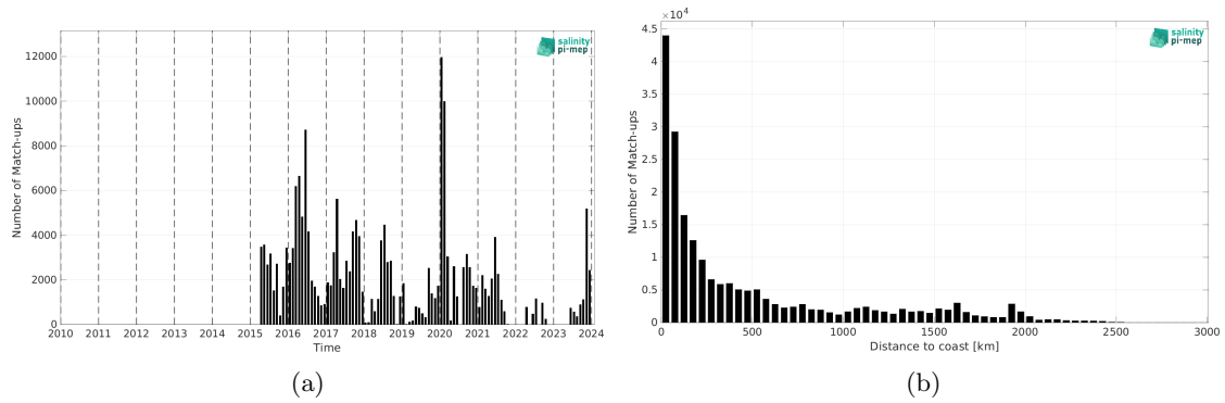
Figure 2: Number of match-ups between TSG (SAMOS) and SMAP SSS L3 v5.0 - Monthly (JPL) SSS as a function of time (a) and as function of the distance to coast (b) over the Tropical Pacific Ocean Pi-MEP region and for the full satellite product period.
