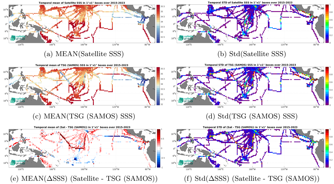
Figure 7: Temporal mean (left) and Std (right) of SSS from SMAP SSS L3 v5.0 - Monthly (JPL) (top), TSG (SAMOS) (middle), and of \Delta SSS (Satellite - TSG (SAMOS)). Only match-up pairs are used to generate these maps.
