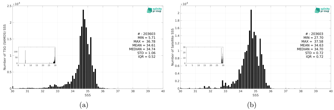
Figure 3: Histograms of SSS from TSG (SAMOS) (a) and SMAP SSS L3 v5.0 - Monthly (JPL) (b) considering all match-up pairs per bins of 0.1 over the Tropical Pacific Ocean Pi-MEP region and for the full satellite product period.
