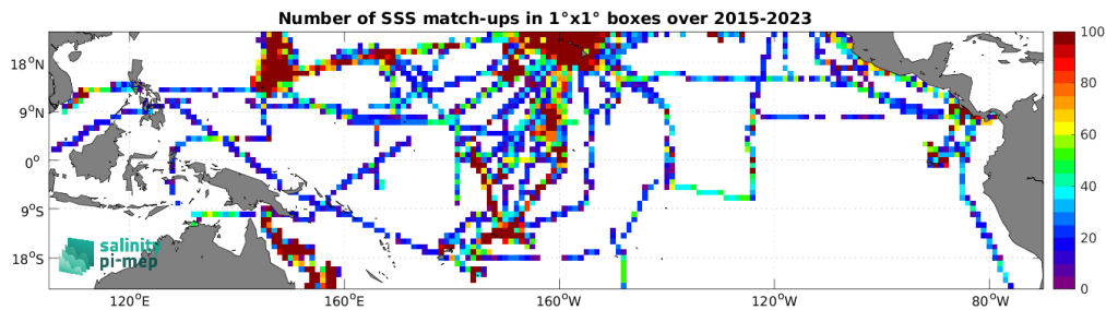
Figure 5: Number of SSS match-ups between TSG (SAMOS) SSS and the SMAP SSS L3 v5.0 - Monthly (JPL) SSS product for the Tropical Pacific Ocean Pi-MEP region over 1^\circ \times 1^\circ boxes and for the full satellite product period.
