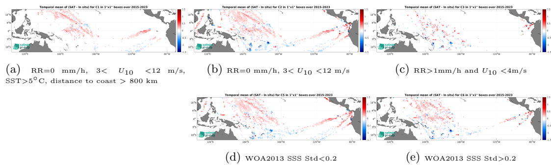
Figure 14: Temporal mean gridded over spatial boxes of size 1^\circ \times 1^\circ of \Delta SSS (SMAP SSS L3 v5.0 - Monthly (JPL) - TSG (LEGOS-DM)) for 5 different subdatasets corresponding to: RR=0 mm/h, 3 < U_{10} < 12 m/s, SST > 5^\circ\text{C} , distance to coast > 800 km (a), RR=0 mm/h, 3 < U_{10} < 12 m/s (b), RR > 1 mm/h and U_{10} < 4 m/s (c), WOA2013 SSS Std < 0.2 (d), WOA2013 SSS Std > 0.2 (e).
