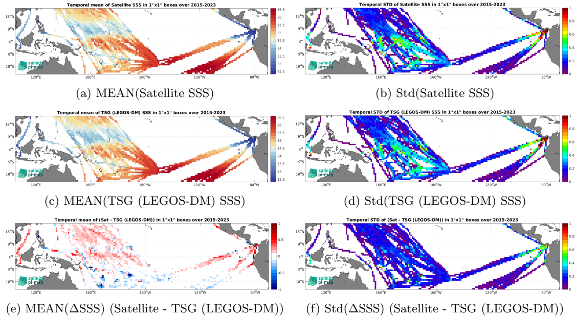
Figure 7: Temporal mean (left) and Std (right) of SSS from SMAP SSS L3 v5.0 - Monthly (JPL) (top), TSG (LEGOS-DM) (middle), and of \Delta SSS (Satellite - TSG (LEGOS-DM)). Only match-up pairs are used to generate these maps.
