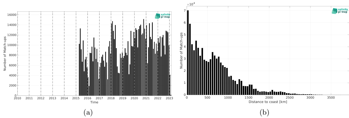
Figure 2: Number of match-ups between TSG (LEGOS-DM) and SMAP SSS L3 v5.0 - Monthly (JPL) SSS as a function of time (a) and as function of the distance to coast (b) over the Tropical Pacific Ocean Pi-MEP region and for the full satellite product period.
