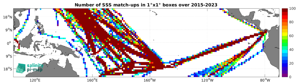
Figure 5: Number of SSS match-ups between TSG (LEGOS-DM) SSS and the SMAP SSS L3 v5.0 - Monthly (JPL) SSS product for the Tropical Pacific Ocean Pi-MEP region over 1^\circ \times 1^\circ boxes and for the full satellite product period.
