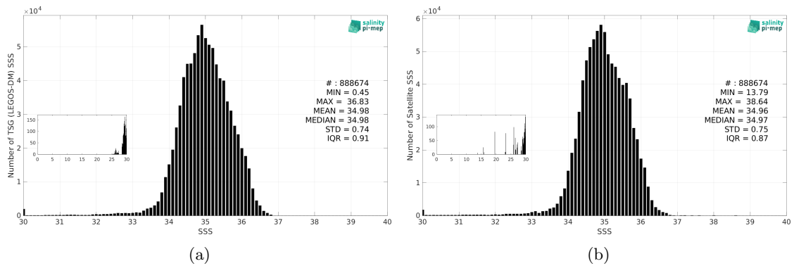
Figure 3: Histograms of SSS from TSG (LEGOS-DM) (a) and SMAP SSS L3 v5.0 - Monthly (JPL) (b) considering all match-up pairs per bins of 0.1 over the Tropical Pacific Ocean Pi-MEP region and for the full satellite product period.
