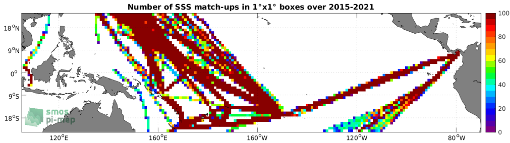
Figure 4: Number of SSS match-ups between TSG (LEGOS-DM) SSS and the SMAP SSS L3 v5.0 - Monthly (JPL) SSS product for the Tropical Pacific Ocean Pi-MEP region over 1^\circ \times 1^\circ boxes and for the full satellite product period.
