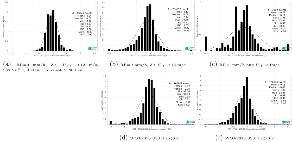
Figure 15: Normalized histogram of \Delta\text{SSS} (SMAP SSS L3 v5.0 - Monthly (JPL) - TSG (GOSUD-Research-vessel)) for 5 different subdatasets corresponding to: RR=0 mm/h, 3 < U_{10} < 12 m/s, SST > 5^\circ\text{C} , distance to coast > 800 km (a), RR=0 mm/h, 3 < U_{10} < 12 m/s (b), RR > 1 mm/h and U_{10} < 4 m/s (c), WOA2013 SSS Std < 0.2 (d), WOA2013 SSS Std > 0.2 (e).
