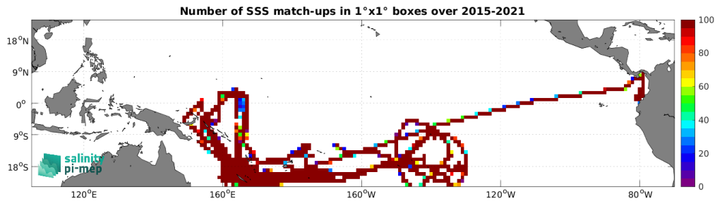
Figure 4: Number of SSS match-ups between TSG (GOSUD-Research-vessel) SSS and the SMAP SSS L3 v5.0 - Monthly (JPL) SSS product for the Tropical Pacific Ocean Pi-MEP region over 1^\circ \times 1^\circ boxes and for the full satellite product period.
