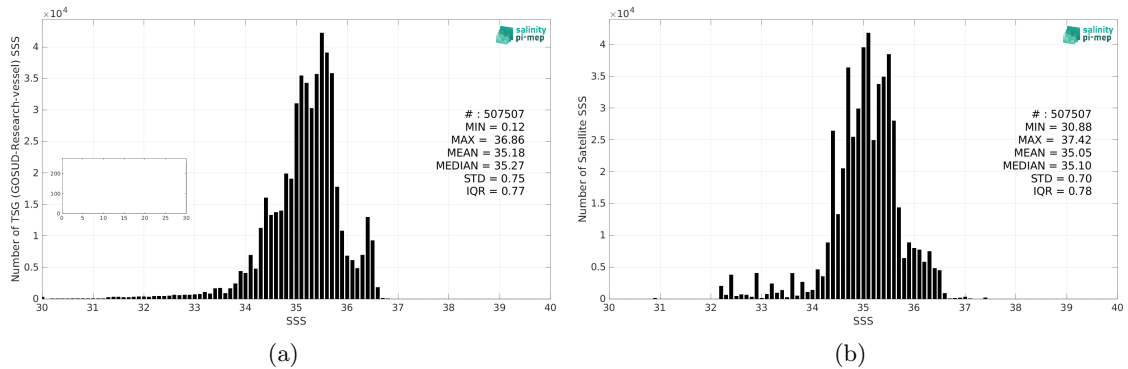
Figure 2: Histograms of SSS from TSG (GOSUD-Research-vessel) (a) and SMAP SSS L3 v5.0 - Monthly (JPL) (b) considering all match-up pairs per bins of 0.1 over the Tropical Pacific Ocean Pi-MEP region and for the full satellite product period.
