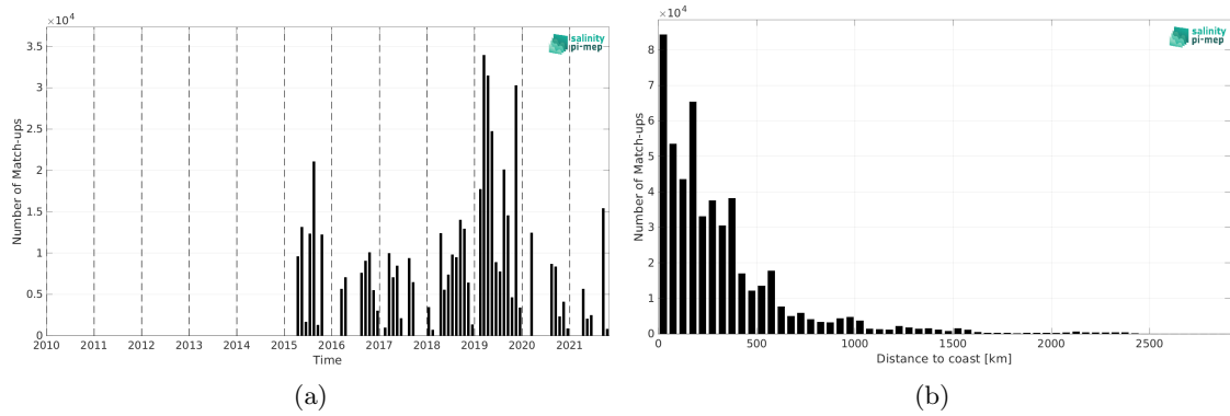
Figure 1: Number of match-ups between TSG (GOSUD-Research-vessel) and SMAP SSS L3 v5.0 - Monthly (JPL) SSS as a function of time (a) and as function of the distance to coast (b) over the Tropical Pacific Ocean Pi-MEP region and for the full satellite product period.
