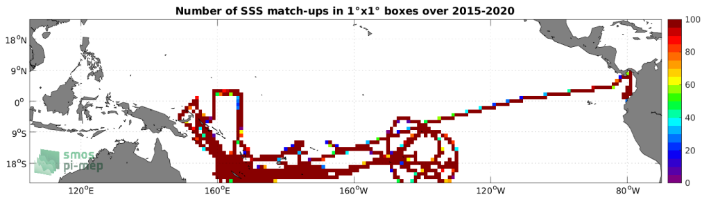
Figure 4: Number of SSS match-ups between TSG (GOSUD-Research-vessel) SSS and the SMAP SSS L3 v5.0 - Monthly (JPL) SSS product for the Tropical Pacific Ocean Pi-MEP region over 1°×1° boxes and for the full satellite product period.
