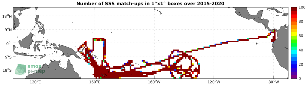
Figure 4: Number of SSS match-ups between TSG (GOSUD-Research-vessel) SSS and the SMAP SSS L3 v5.0 - Monthly (JPL) SSS product for the Tropical Pacific Ocean Pi-MEP region over 1^\circ \times 1^\circ boxes and for the full satellite product period.
