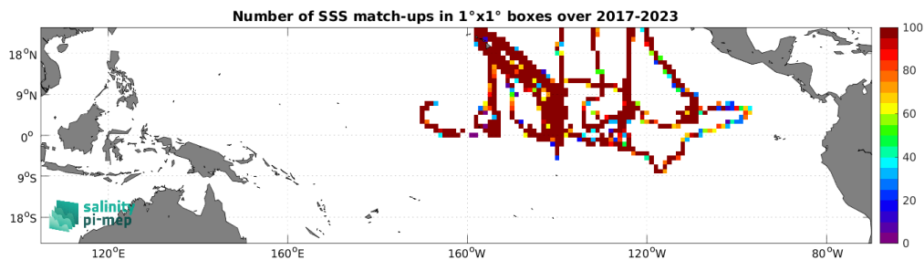
Figure 5: Number of SSS match-ups between Saildrone SSS and the SMAP SSS L3 v5.0 - Monthly (JPL) SSS product for the Tropical Pacific Ocean Pi-MEP region over 1^\circ \times 1^\circ boxes and for the full satellite product period.
