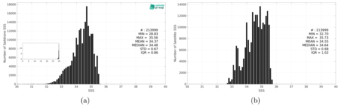
Figure 3: Histograms of SSS from Saildrone (a) and SMAP SSS L3 v5.0 - Monthly (JPL) (b) considering all match-up pairs per bins of 0.1 over the Tropical Pacific Ocean Pi-MEP region and for the full satellite product period.
