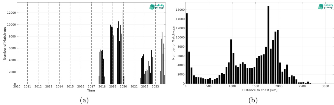
Figure 2: Number of match-ups between Saildrone and SMAP SSS L3 v5.0 - Monthly (JPL) SSS as a function of time (a) and as function of the distance to coast (b) over the Tropical Pacific Ocean Pi-MEP region and for the full satellite product period.
