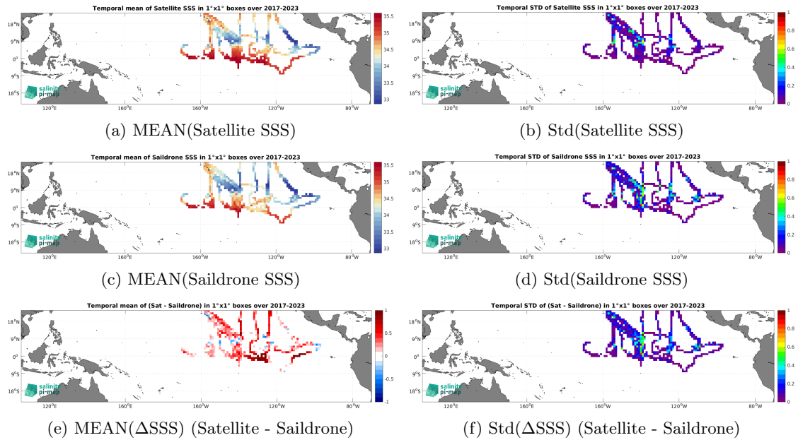
Figure 7: Temporal mean (left) and Std (right) of SSS from SMAP SSS L3 v5.0 - Monthly (JPL) (top), Saildrone (middle), and of \Delta SSS (Satellite - Saildrone). Only match-up pairs are used to generate these maps.
