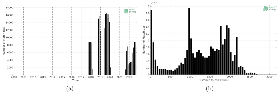
Figure 1: Number of match-ups between Saildrone and SMAP SSS L3 v5.0 - Monthly (JPL) SSS as a function of time (a) and as function of the distance to coast (b) over the Tropical Pacific Ocean Pi-MEP region and for the full satellite product period.
