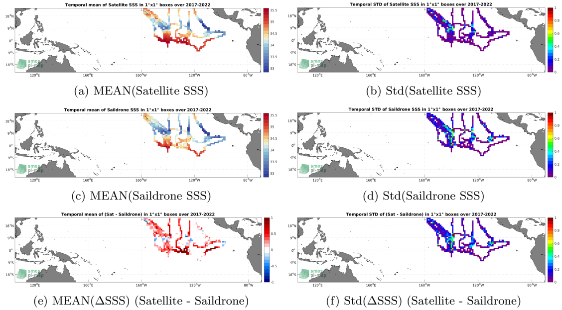
Figure 6: Temporal mean (left) and Std (right) of SSS from SMAP SSS L3 v5.0 - Monthly (JPL) (top), Saildrone (middle), and of \Delta SSS (Satellite - Saildrone). Only match-up pairs are used to generate these maps.
