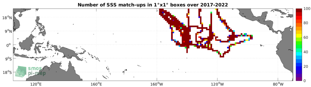
Figure 4: Number of SSS match-ups between Saildrone SSS and the SMAP SSS L3 v5.0 - Monthly (JPL) SSS product for the Tropical Pacific Ocean Pi-MEP region over 1^\circ \times 1^\circ boxes and for the full satellite product period.
