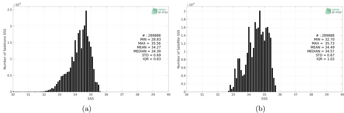
Figure 2: Histograms of SSS from Saildrone (a) and SMAP SSS L3 v5.0 - Monthly (JPL) (b) considering all match-up pairs per bins of 0.1 over the Tropical Pacific Ocean Pi-MEP region and for the full satellite product period.
