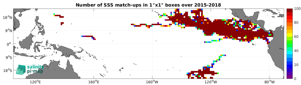
Figure 4: Number of SSS match-ups between Surface drifters SSS and the SMAP SSS L3 v5.0 - Monthly (JPL) SSS product for the Tropical Pacific Ocean Pi-MEP region over 1^\circ \times 1^\circ boxes and for the full satellite product period.
