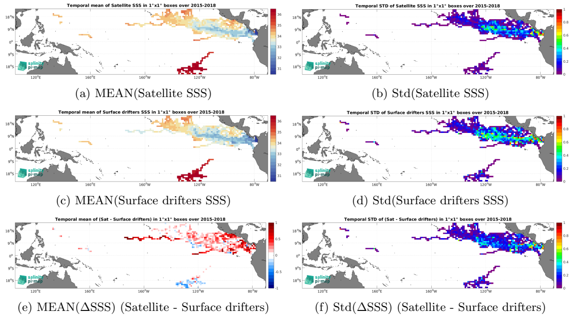
Figure 6: Temporal mean (left) and Std (right) of SSS from SMAP SSS L3 v5.0 - Monthly (JPL) (top), Surface drifters (middle), and of \Delta SSS (Satellite - Surface drifters). Only match-up pairs are used to generate these maps.
