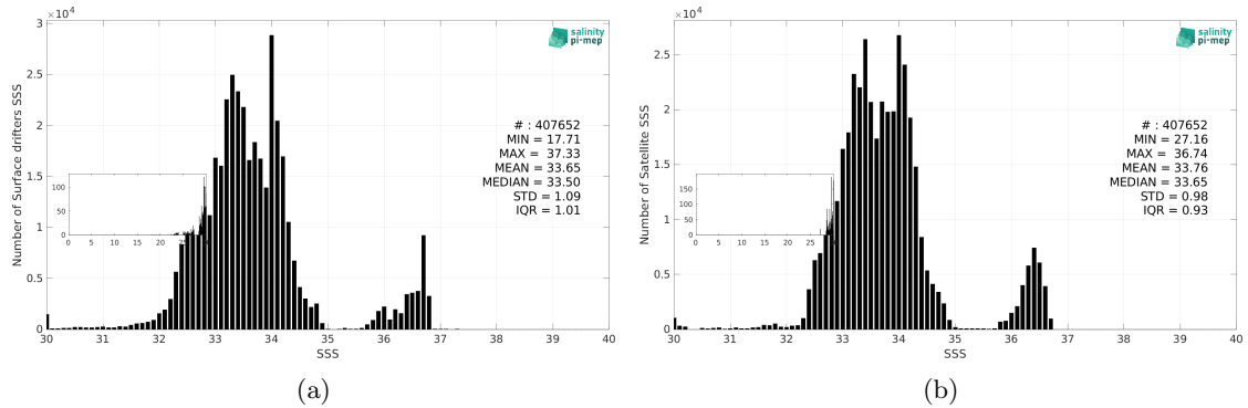
Figure 3: Histograms of SSS from Surface drifters (a) and SMAP SSS L3 v5.0 - Monthly (JPL) (b) considering all match-up pairs per bins of 0.1 over the Tropical Pacific Ocean Pi-MEP region and for the full satellite product period.
