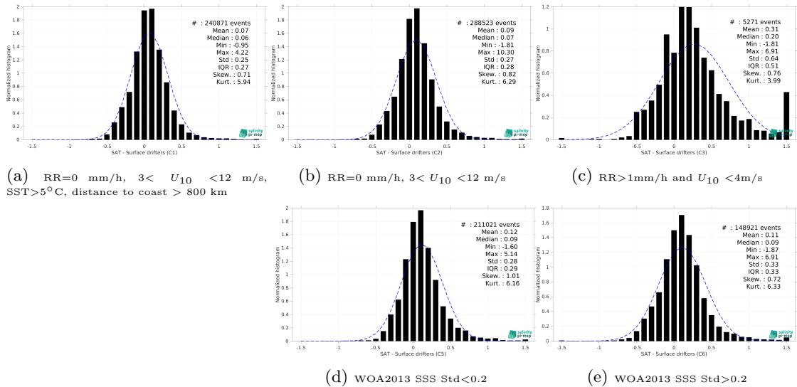
Figure 14: Normalized histogram of \Delta SSS (SMAP SSS L3 v5.0 - Monthly (JPL) - Surface drifters) for 5 different subdatasets corresponding to: RR=0 mm/h, 3 < U_{10} < 12 m/s, SST > 5^\circ C , distance to coast > 800 km (a), RR=0 mm/h, 3 < U_{10} < 12 m/s (b), RR > 1 mm/h and U_{10} < 4 m/s (c), WOA2013 SSS Std <0.2 (d), WOA2013 SSS Std >0.2 (e).
