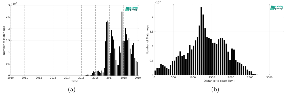
Figure 2: Number of match-ups between Surface drifters and SMAP SSS L3 v5.0 - Monthly (JPL) SSS as a function of time (a) and as function of the distance to coast (b) over the Tropical Pacific Ocean Pi-MEP region and for the full satellite product period.
