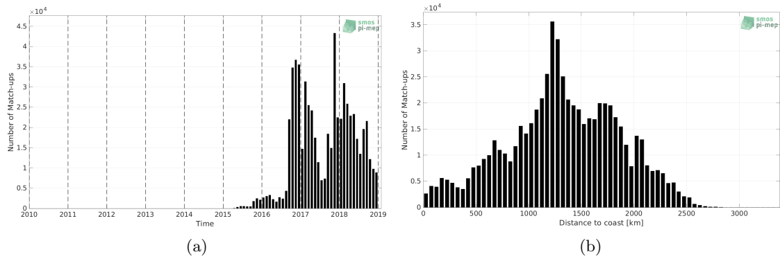
Figure 1: Number of match-ups between Surface drifters and SMAP SSS L3 v5.0 - Monthly (JPL) SSS as a function of time (a) and as function of the distance to coast (b) over the Tropical Pacific Ocean Pi-MEP region and for the full satellite product period.
