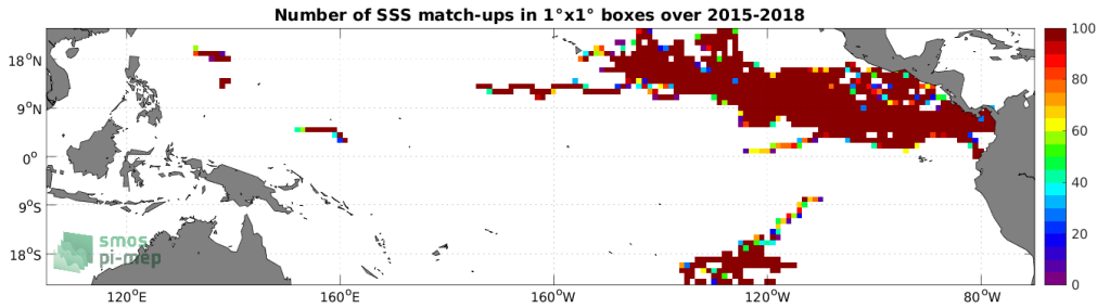
Figure 3: Number of SSS match-ups between Surface drifters SSS and the SMAP SSS L3 v5.0 - Monthly (JPL) SSS product for the Tropical Pacific Ocean Pi-MEP region over 1^\circ \times 1^\circ boxes and for the full satellite product period.
