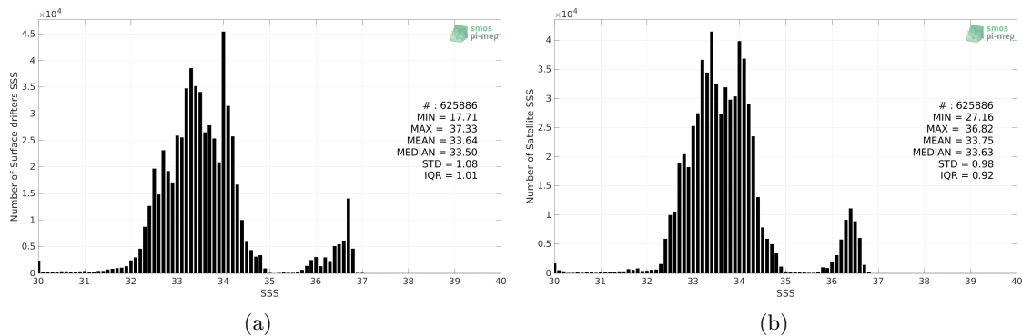
Figure 2: Histograms of SSS from Surface drifters (a) and SMAP SSS L3 v5.0 - Monthly (JPL) (b) considering all match-up pairs per bins of 0.1 over the Tropical Pacific Ocean Pi-MEP region and for the full satellite product period.
