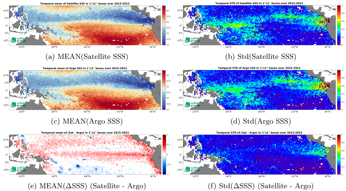
Figure 7: Temporal mean (left) and Std (right) of SSS from SMAP SSS L3 v5.0 - Monthly (JPL) (top), Argo (middle), and of \Delta SSS (Satellite - Argo). Only match-up pairs are used to generate these maps.
