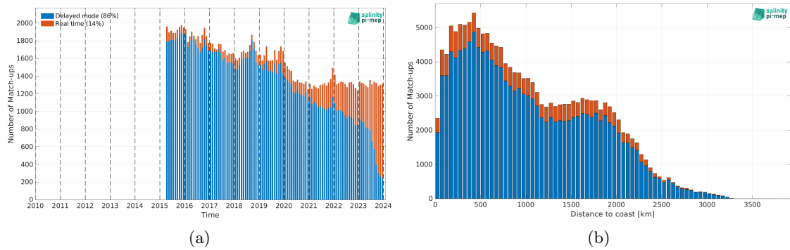
Figure 2: Number of match-ups between Argo and SMAP SSS L3 v5.0 - Monthly (JPL) SSS as a function of time (a) and as function of the distance to coast (b) over the Tropical Pacific Ocean Pi-MEP region and for the full satellite product period.
