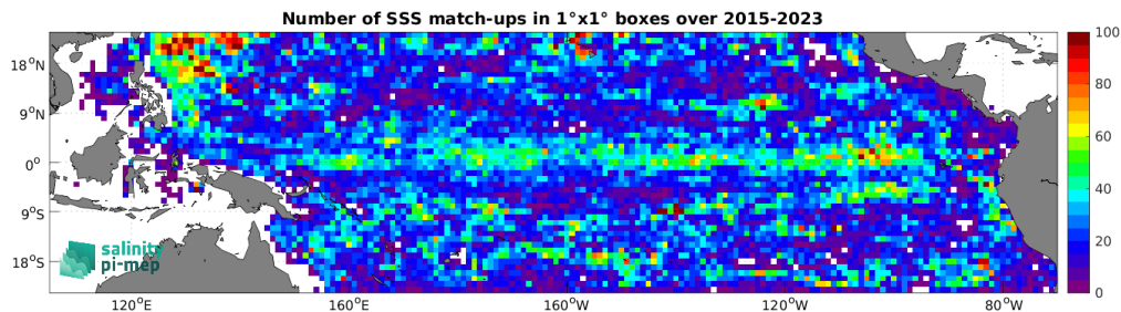
Figure 5: Number of SSS match-ups between Argo SSS and the SMAP SSS L3 v5.0 - Monthly (JPL) SSS product for the Tropical Pacific Ocean Pi-MEP region over 1^\circ \times 1^\circ boxes and for the full satellite product period.
