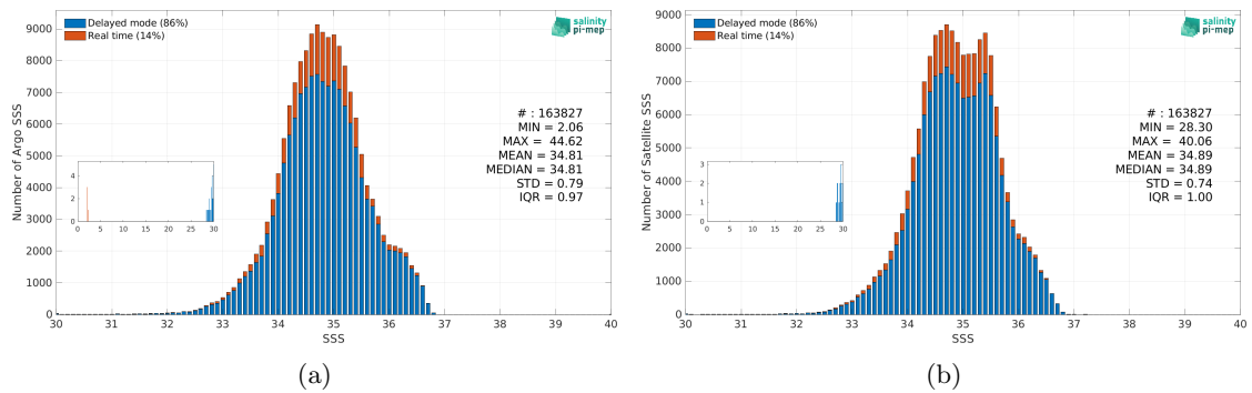
Figure 3: Histograms of SSS from Argo (a) and SMAP SSS L3 v5.0 - Monthly (JPL) (b) considering all match-up pairs per bins of 0.1 over the Tropical Pacific Ocean Pi-MEP region and for the full satellite product period.
