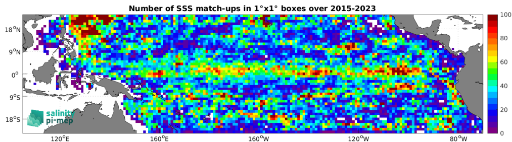
Figure 4: Number of SSS match-ups between Argo SSS and the SMAP SSS L3 v5.0 - Monthly (JPL) SSS product for the Tropical Pacific Ocean Pi-MEP region over 1^\circ \times 1^\circ boxes and for the full satellite product period.
