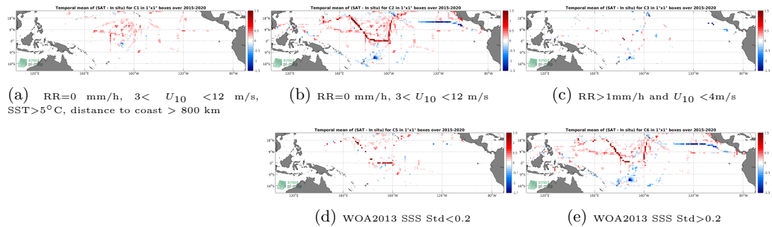
Figure 12: Temporal mean gridded over spatial boxes of size 1^\circ \times 1^\circ of \Delta SSS (SMAP-L3-JPL-V4.3-8DAY-RUNNING-60KM - TSG-SAMOS) for 5 different subdatasets corresponding to: RR=0 mm/h, 3 < U_{10} < 12 m/s, SST > 5^\circ\text{C} , distance to coast > 800 km (a), RR=0 mm/h, 3 < U_{10} < 12 m/s (b), RR > 1\text{mm/h} and U_{10} < 4\text{m/s} (c), WOA2013 SSS Std < 0.2 (d), WOA2013 SSS Std > 0.2 (e).
