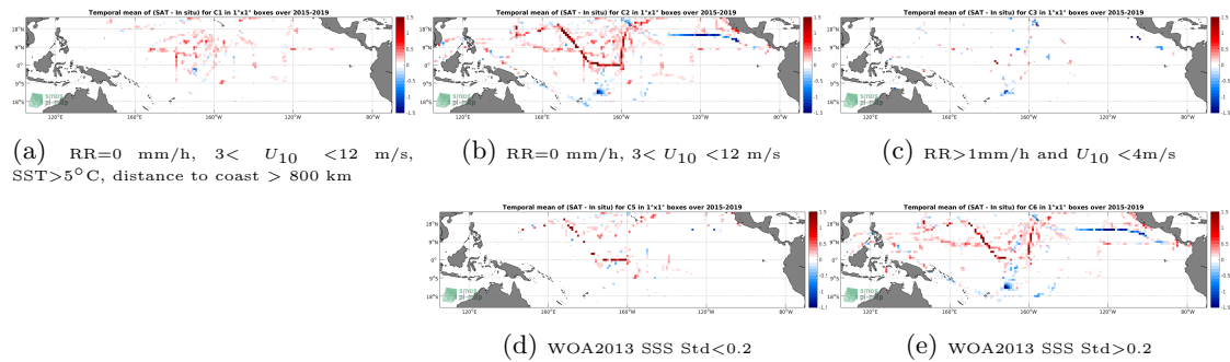
Figure 12: Temporal mean gridded over spatial boxes of size 1^\circ \times 1^\circ of \Delta SSS (SMAP-L3-JPL-V4.3-8DAY-RUNNING-60KM - TSG-SAMOS) for 5 different subdatasets corresponding to:RR=0 mm/h, 3 < U_{10} < 12 m/s, SST > 5^\circ C , distance to coast > 800 km (a), RR=0 mm/h, 3 < U_{10} < 12 m/s (b), RR >1 mm/h and U_{10} < 4 m/s (c), WOA2013 SSS Std <0.2 (d), WOA2013 SSS Std >0.2 (e).
