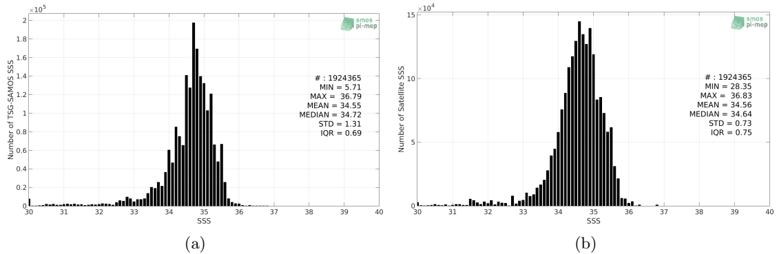
Figure 2: Histograms of SSS from TSG-SAMOS (a) and SMAP-L3-JPL-V4.3-8DAY-RUNNING-60KM (b) considering all match-up pairs per bins of 0.1 over the Tropical Pacific Ocean Pi-MEP region and for the full satellite product period.
