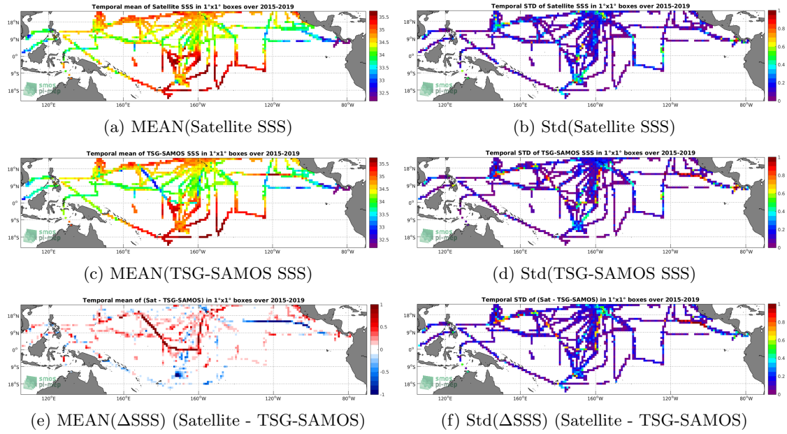
Figure 6: Temporal mean (left) and Std (right) of SSS from SMAP-L3-JPL-V4.3-8DAY-RUNNING-60KM (top), TSG-SAMOS (middle), and of \Delta SSS (Satellite - TSG-SAMOS). Only match-up pairs are used to generate these maps.
