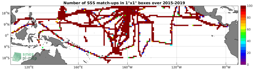
Figure 4: Number of SSS match-ups between TSG-SAMOS SSS and the SMAP-L3-JPL-V4.3-8DAY-RUNNING-60KM SSS product for the Tropical Pacific Ocean Pi-MEP region over 1^\circ \times 1^\circ boxes and for the full satellite product period.
