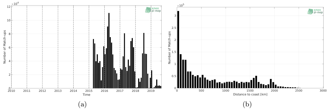
Figure 1: Number of match-ups between TSG-SAMOS and SMAP-L3-JPL-V4.3-8DAY-RUNNING-60KM SSS as a function of time (a) and as function of the distance to coast (b) over the Tropical Pacific Ocean Pi-MEP region and for the full satellite product period.
