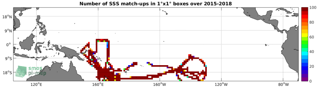
Figure 4: Number of SSS match-ups between TSG-GOSUD-Research-vessel SSS and the SMAP-L3-JPL-V4.3-8DAY-RUNNING-60KM SSS product for the Tropical Pacific Ocean Pi-MEP region over 1°x1° boxes and for the full satellite product period.
