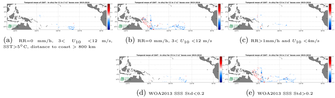
Figure 12: Temporal mean gridded over spatial boxes of size 1^{\circ}\times 1^{\circ} of \Delta SSS (SMAP-L3-JPL-V4.3-8DAY-RUNNING-60KM - TSG-GOSUD-Research-vessel) for 5 different subdatasets corresponding to:RR=0 mm/h, 3 < U_{10} < 12 m/s, SST >5^{\circ}\text{C} , distance to coast > 800 km (a), RR=0 mm/h, 3 < U_{10} < 12 m/s (b), RR >1 mm/h and U_{10} < 4 m/s (c), WOA2013 SSS Std <0.2 (d), WOA2013 SSS Std >0.2 (e).
