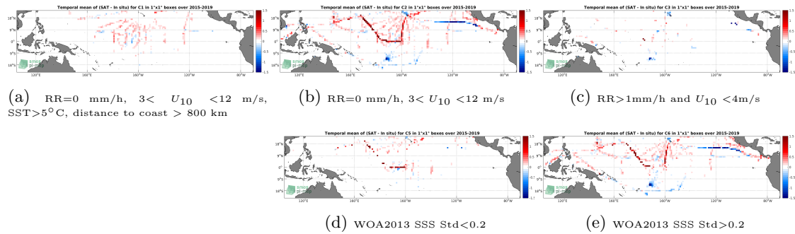
Figure 12: Temporal mean gridded over spatial boxes of size 1^\circ \times 1^\circ of \Delta SSS (SMAP-L3-JPL-V4.3-MONTHLY-60KM - TSG-SAMOS) for 5 different subdatasets corresponding to: RR=0 mm/h, 3 < U_{10} < 12 m/s, SST > 5^\circ\text{C} , distance to coast > 800 km (a), RR=0 mm/h, 3 < U_{10} < 12 m/s (b), RR > 1 mm/h and U_{10} < 4 m/s (c), WOA2013 SSS Std < 0.2 (d), WOA2013 SSS Std > 0.2 (e).
