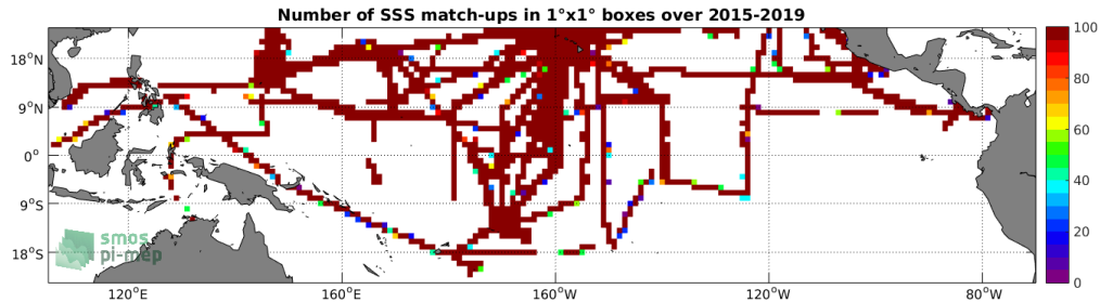
Figure 4: Number of SSS match-ups between TSG-SAMOS SSS and the SMAP-L3-JPL-V4.3-MONTHLY-60KM SSS product for the Tropical Pacific Ocean Pi-MEP region over 1°x1° boxes and for the full satellite product period.
