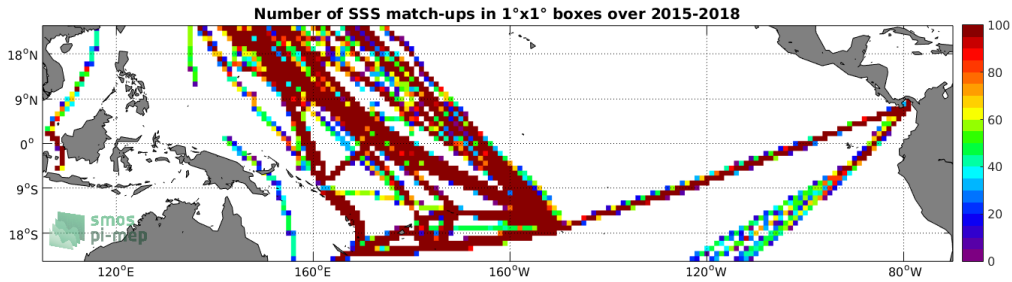
Figure 4: Number of SSS match-ups between TSG-LEGOS-DM SSS and the SMAP-L3-JPL-V4.3-MONTHLY-60KM SSS product for the Tropical Pacific Ocean Pi-MEP region over 1^\circ \times 1^\circ boxes and for the full satellite product period.
