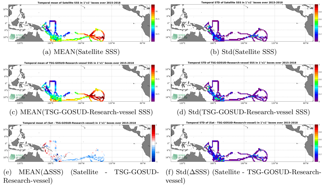
Figure 6: Temporal mean (left) and Std (right) of SSS from SMAP-L3-JPL-V4.3-MONTHLY-60KM (top), TSG-GOSUD-Research-vessel (middle), and of \Delta SSS (Satellite - TSG-GOSUD-Research-vessel). Only match-up pairs are used to generate these maps.
