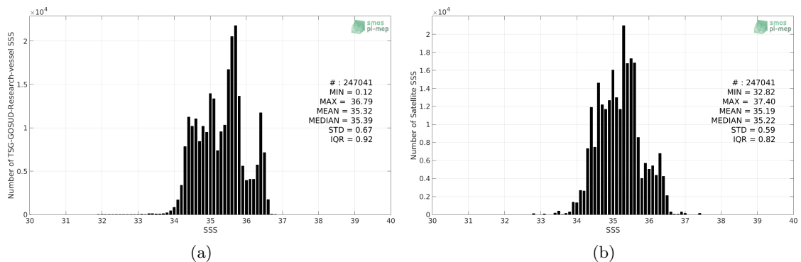
Figure 2: Histograms of SSS from TSG-GOSUD-Research-vessel (a) and SMAP-L3-JPL-V4.3-MONTHLY-60KM (b) considering all match-up pairs per bins of 0.1 over the Tropical Pacific Ocean Pi-MEP region and for the full satellite product period.
