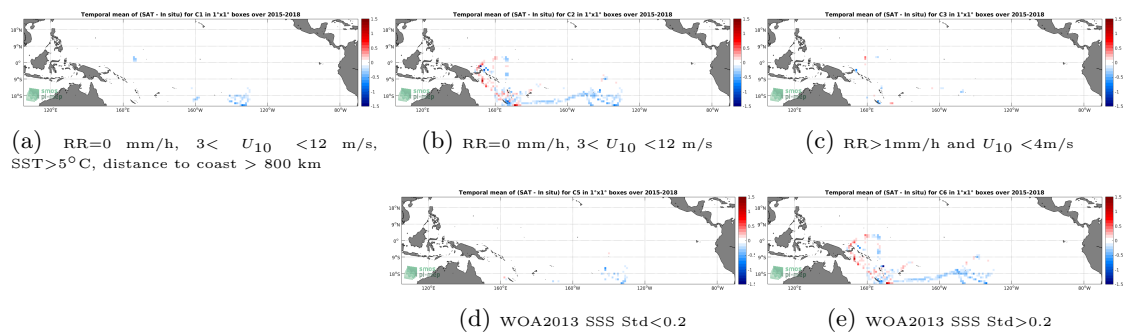
Figure 12: Temporal mean gridded over spatial boxes of size 1^\circ \times 1^\circ of \Delta SSS (SMAP-L3-JPL-V4.3-MONTHLY-60KM - TSG-GOSUD-Research-vessel) for 5 different subdatasets corresponding to: RR=0 mm/h, 3 < U_{10} < 12 m/s, SST > 5°C, distance to coast > 800 km (a), RR=0 mm/h, 3 < U_{10} < 12 m/s (b), RR > 1mm/h and U_{10} < 4 m/s (c), WOA2013 SSS Std < 0.2 (d), WOA2013 SSS Std > 0.2 (e).
