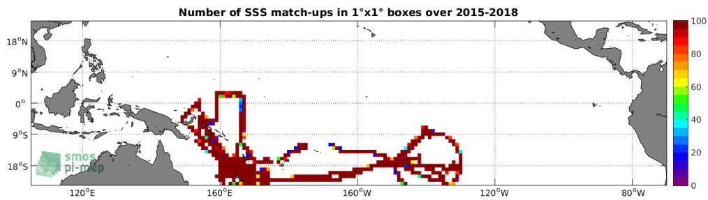
Figure 4: Number of SSS match-ups between TSG-GOSUD-Research-vessel SSS and the SMAP-L3-JPL-V4.3-MONTHLY-60KM SSS product for the Tropical Pacific Ocean Pi-MEP region over 1^\circ \times 1^\circ boxes and for the full satellite product period.
