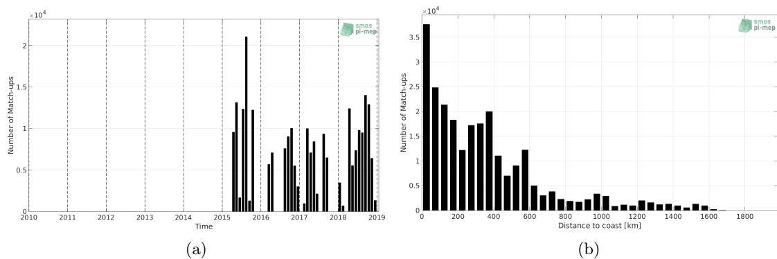
Figure 1: Number of match-ups between TSG-GOSUD-Research-vessel and SMAP-L3-JPL-V4.3-MONTHLY-60KM SSS as a function of time (a) and as function of the distance to coast (b) over the Tropical Pacific Ocean Pi-MEP region and for the full satellite product period.
