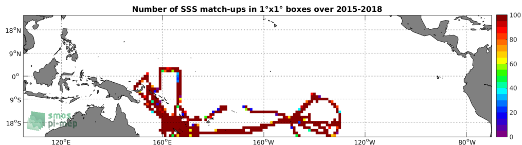
Figure 4: Number of SSS match-ups between TSG-GOSUD-Research-vessel SSS and the SMAP-L3-JPL-V4.3-MONTHLY-60KM SSS product for the Tropical Pacific Ocean Pi-MEP region over 1°x1° boxes and for the full satellite product period.
