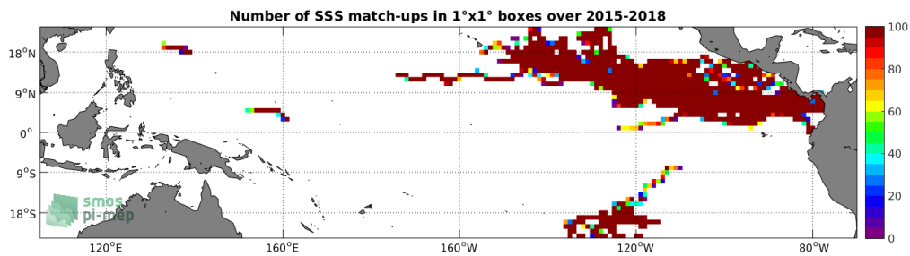
Figure 3: Number of SSS match-ups between Surface drifters SSS and the SMAP-L3-JPL-V4.3-MONTHLY-60KM SSS product for the Tropical Pacific Ocean Pi-MEP region over 1°x1° boxes and for the full satellite product period.
