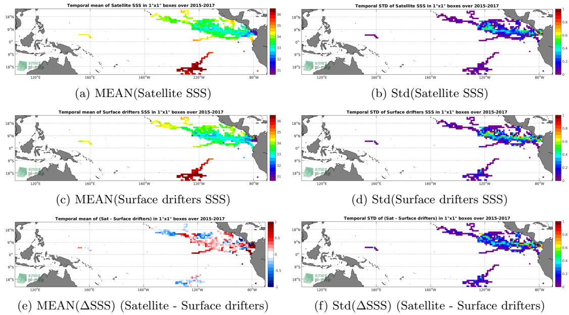
Figure 5: Temporal mean (left) and Std (right) of SSS from SMAP-L3-JPL-V4.3-MONTHLY-60KM (top), Surface drifters (middle), and of \Delta SSS (Satellite - Surface drifters). Only match-up pairs are used to generate these maps.
