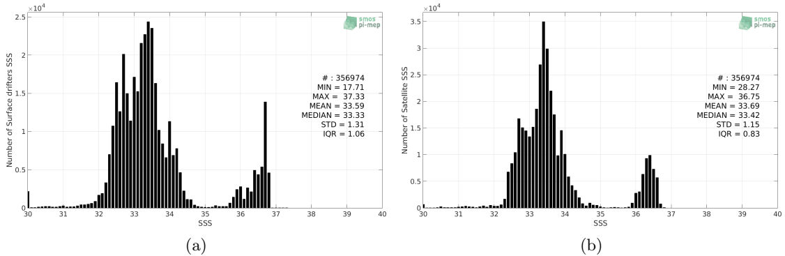
Figure 2: Histograms of SSS from Surface drifters (a) and SMAP-L3-JPL-V4.3-MONTHLY-60KM (b) considering all match-up pairs per bins of 0.1 over the Tropical Pacific Ocean Pi-MEP region and for the full satellite product period.
