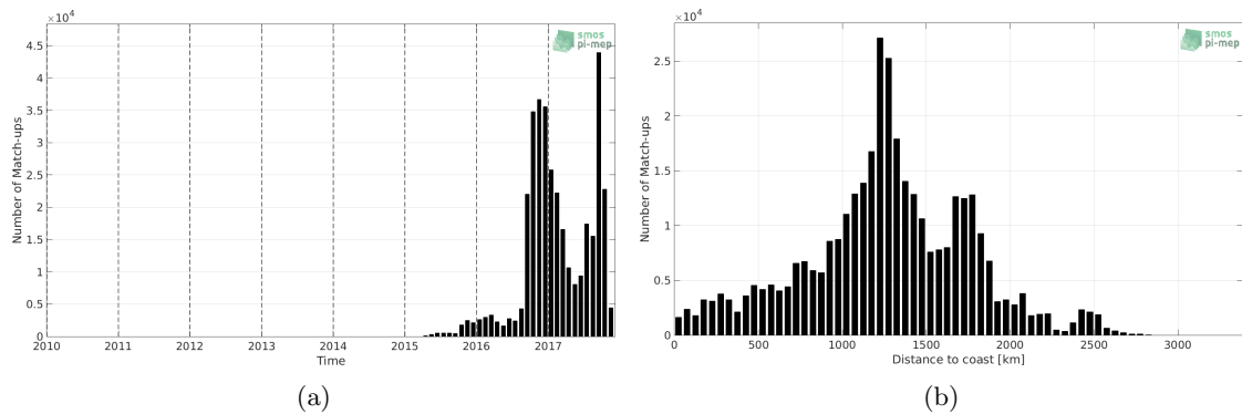
Figure 1: Number of match-ups between Surface drifters and SMAP-L3-JPL-V4.3-MONTHLY-60KM SSS as a function of time (a) and as function of the distance to coast (b) over the Tropical Pacific Ocean Pi-MEP region and for the full satellite product period.
