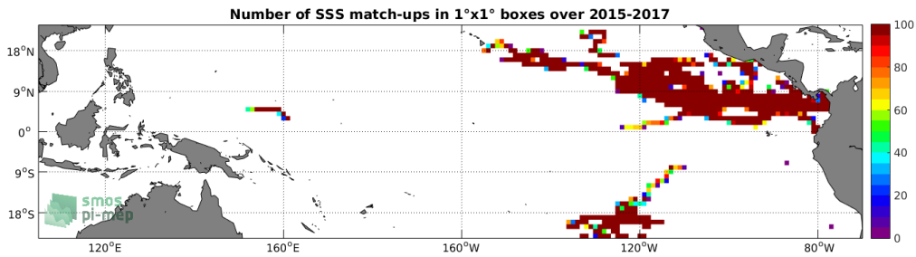
Figure 3: Number of SSS match-ups between Surface drifters SSS and the SMAP-L3-JPL-V4.3-MONTHLY-60KM SSS product for the Tropical Pacific Ocean Pi-MEP region over 1^\circ \times 1^\circ boxes and for the full satellite product period.
