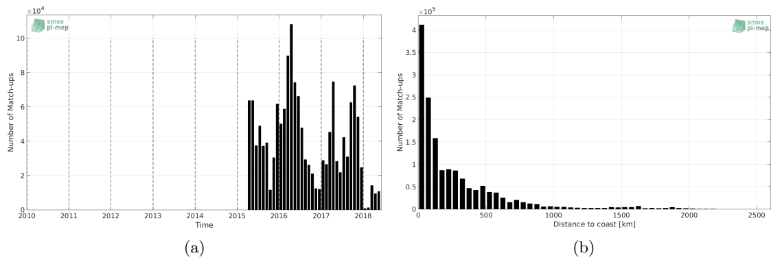
Figure 1: Number of match-ups between TSG-SAMOS and SMAP-L3-JPL-V4-8DAY-RUNNING-60KM SSS as a function of time (a) and as function of the distance to coast (b) over the Tropical Pacific Ocean Pi-MEP region and for the full satellite product period.
