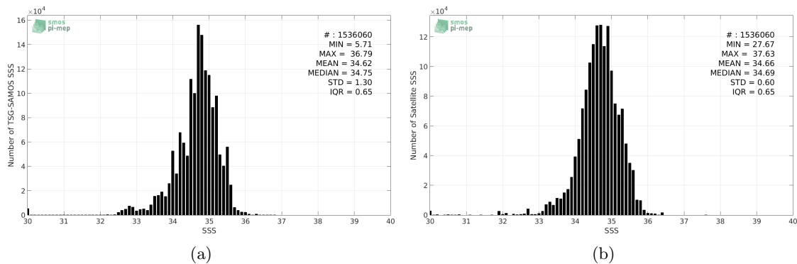
Figure 2: Histograms of SSS from TSG-SAMOS (a) and SMAP-L3-JPL-V4-8DAY-RUNNING-60KM (b) considering all match-up pairs per bins of 0.1 over the Tropical Pacific Ocean Pi-MEP region and for the full satellite product period.
