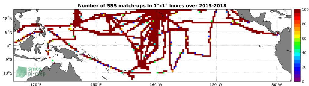
Figure 4: Number of SSS match-ups between TSG-SAMOS SSS and the SMAP-L3-JPL-V4-8DAY-RUNNING-60KM SSS product for the Tropical Pacific Ocean Pi-MEP region over 1^\circ \times 1^\circ boxes and for the full satellite product period.
