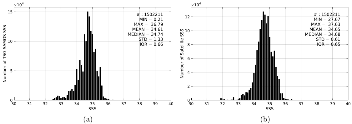
Figure 2: Histograms of SSS from TSG-SAMOS (a) and SMAP-L3-JPL-V4-8DAY-RUNNING-60KM (b) considering all match-up pairs per bins of 0.1 over the Tropical Pacific Ocean Pi-MEP region and for the full satellite product period.
