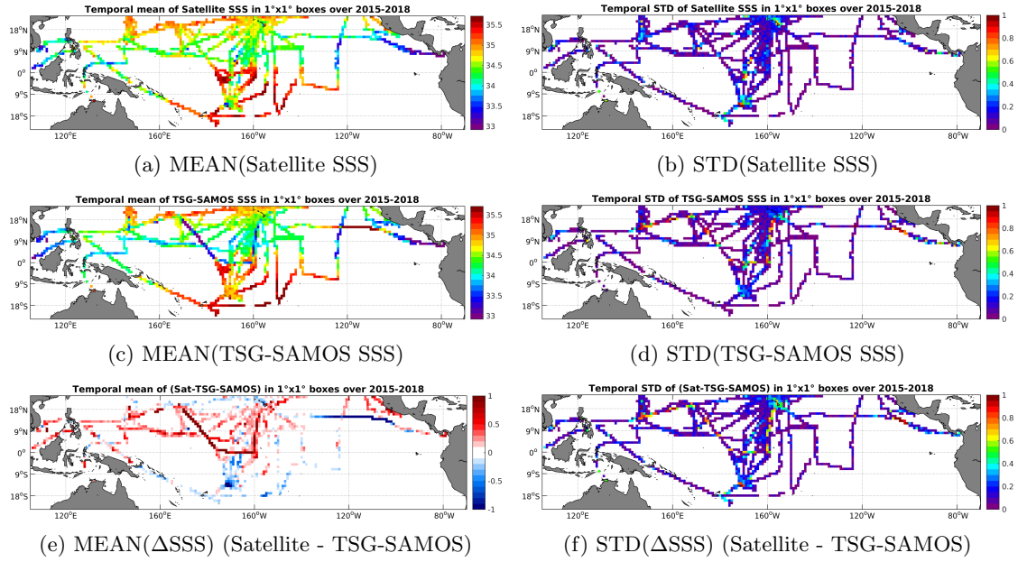
Figure 6: Temporal mean (left) and STD (right) of SSS from SMAP-L3-JPL-V4-8DAY-RUNNING-60KM (top), TSG-SAMOS (middle), and of \Delta SSS (Satellite - TSG-SAMOS). Only match-up pairs are used to generate these maps.
