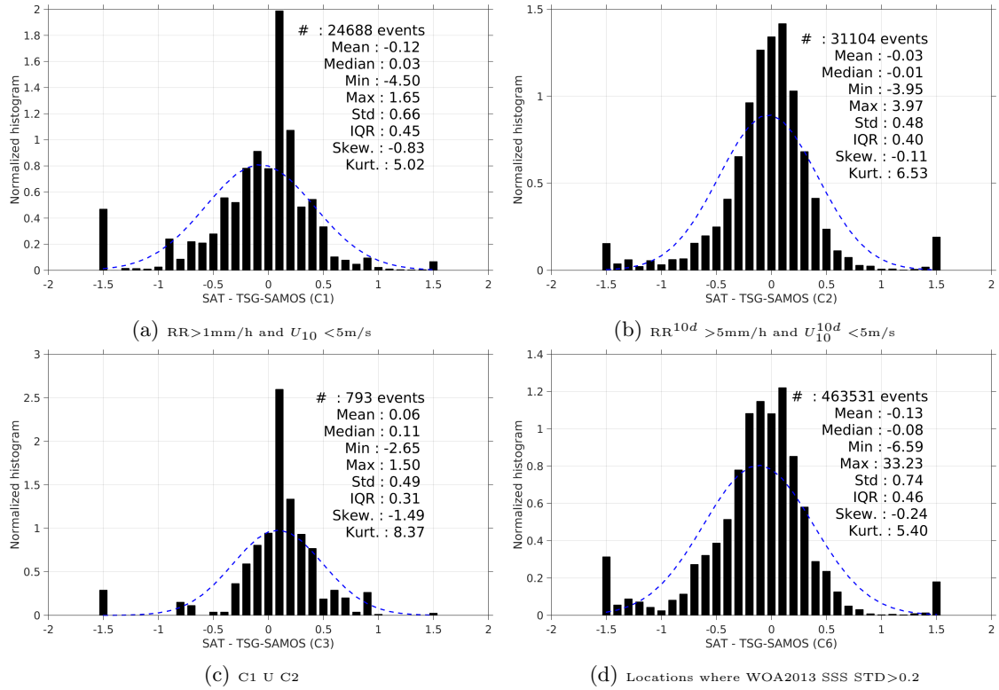
Figure 13: Normalized histogram of \Delta SSS (SMAP-L3-JPL-V4-8DAY-RUNNING-60KM - TSG-SAMOS) for 6 different subdatasets corresponding to: RR > 1\text{mm/h} and U_{10} < 5\text{m/s} (a), RR^{10d} > 5\text{mm/h} and U_{10}^{10d} < 5\text{m/s} (b), C1 U C2 (c), Locations where WOA2013 SSS STD > 0.2 (d).
