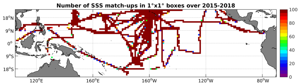
Figure 4: Number of SSS match-ups between TSG-SAMOS SSS and the SMAP-L3-JPL-V4-8DAY-RUNNING-60KM SSS product for the Tropical Pacific Ocean Pi-MEP region over 1^\circ \times 1^\circ boxes and for the full satellite product period.
