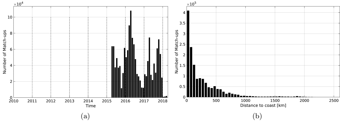
Figure 1: Number of match-ups between TSG-SAMOS and SMAP-L3-JPL-V4-8DAY-RUNNING-60KM SSS as a function of time (a) and as function of the distance to coast (b) over the Tropical Pacific Ocean Pi-MEP region and for the full satellite product period.
