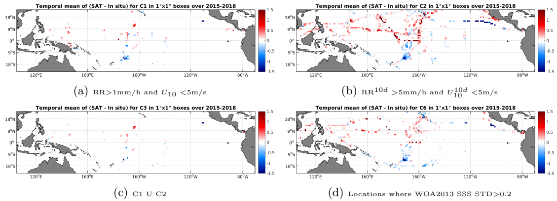
Figure 12: Temporal mean gridded over spatial boxes of size 1^\circ \times 1^\circ of \Delta SSS (SMAP-L3-JPL-V4-8DAY-RUNNING-60KM - TSG-SAMOS) for 4 different subdatasets corresponding to: RR > 1\text{mm/h} and U_{10} < 5\text{m/s} (a), RR^{10d} > 5\text{mm/h} and U_{10}^{10d} < 5\text{m/s} (b), C1 U C2 (c), Locations where WOA2013 SSS STD > 0.2 (d).
