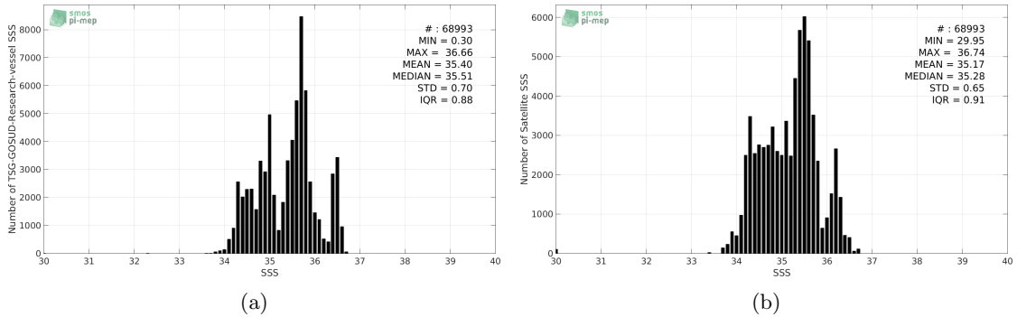
Figure 2: Histograms of SSS from TSG-GOSUD-Research-vessel (a) and SMAP-L3-JPL-V4-8DAY-RUNNING-60KM (b) considering all match-up pairs per bins of 0.1 over the Tropical Pacific Ocean Pi-MEP region and for the full satellite product period.
