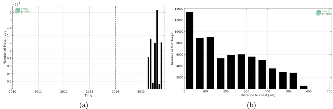
Figure 1: Number of match-ups between TSG-GOSUD-Research-vessel and SMAP-L3-JPL-V4-8DAY-RUNNING-60KM SSS as a function of time (a) and as function of the distance to coast (b) over the Tropical Pacific Ocean Pi-MEP region and for the full satellite product period.
