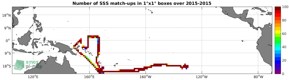
Figure 4: Number of SSS match-ups between TSG-GOSUD-Research-vessel SSS and the SMAP-L3-JPL-V4-8DAY-RUNNING-60KM SSS product for the Tropical Pacific Ocean Pi-MEP region over 1°x1° boxes and for the full satellite product period.
