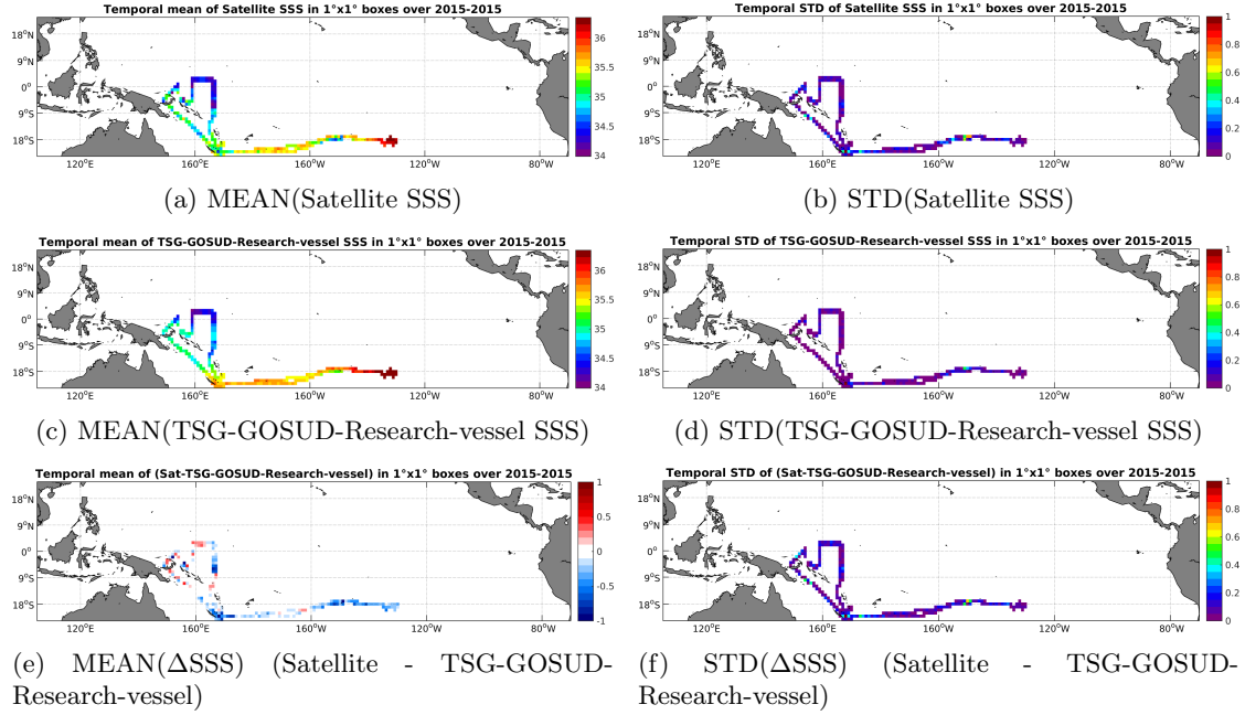
Figure 6: Temporal mean (left) and STD (right) of SSS from SMAP-L3-JPL-V4-8DAY-RUNNING-60KM (top), TSG-GOSUD-Research-vessel (middle), and of \Delta SSS (Satellite - TSG-GOSUD-Research-vessel). Only match-up pairs are used to generate these maps.
