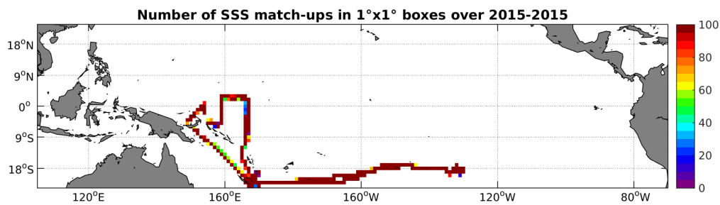
Figure 4: Number of SSS match-ups between TSG-GOSUD-Research-vessel SSS and the SMAP-L3-JPL-V4-8DAY-RUNNING-60KM SSS product for the Tropical Pacific Ocean Pi-MEP region over 1^\circ \times 1^\circ boxes and for the full satellite product period.
