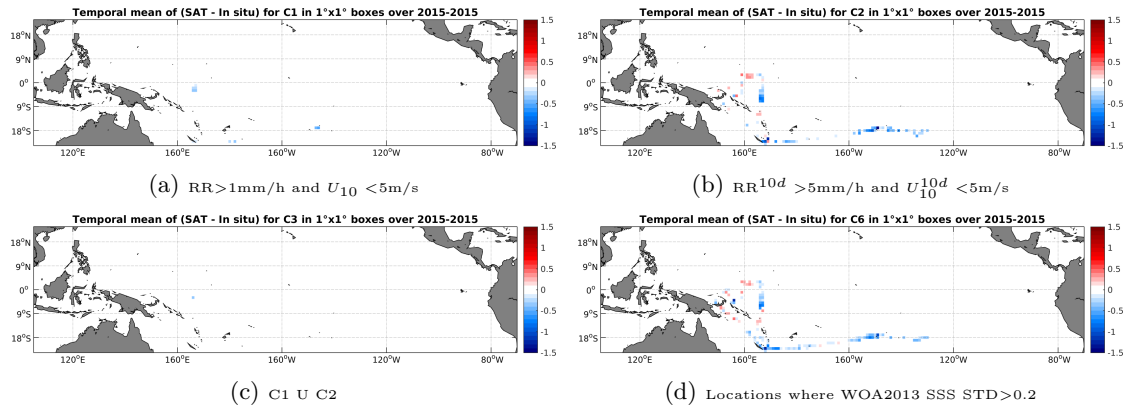
Figure 12: Temporal mean gridded over spatial boxes of size 1^\circ \times 1^\circ of \Delta SSS (SMAP-L3-JPL-V4-8DAY-RUNNING-60KM - TSG-GOSUD-Research-vessel) for 4 different subdatasets corresponding to: RR > 1\text{mm/h} and U_{10} < 5\text{m/s} (a), RR^{10d} > 5\text{mm/h} and U_{10}^{10d} < 5\text{m/s} (b), C1 U C2 (c), Locations where WOA2013 SSS STD > 0.2 (d).
