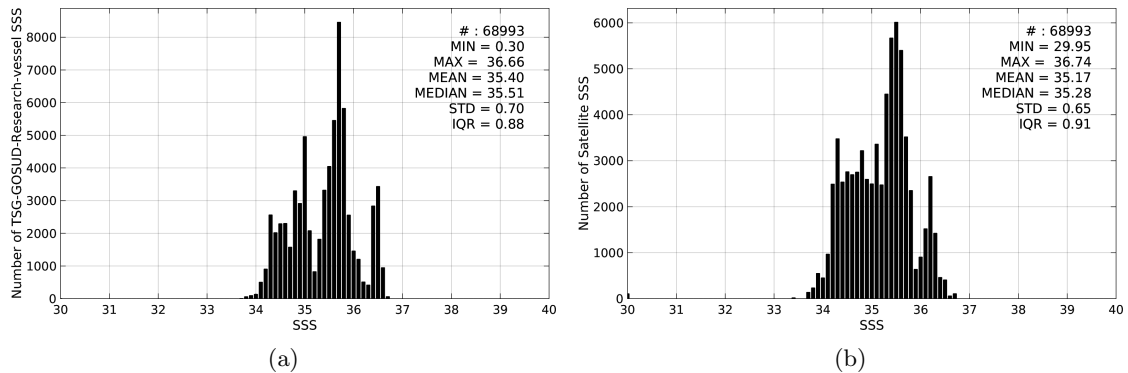
Figure 2: Histograms of SSS from TSG-GOSUD-Research-vessel (a) and SMAP-L3-JPL-V4-8DAY-RUNNING-60KM (b) considering all match-up pairs per bins of 0.1 over the Tropical Pacific Ocean Pi-MEP region and for the full satellite product period.
