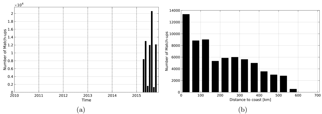
Figure 1: Number of match-ups between TSG-GOSUD-Research-vessel and SMAP-L3-JPL-V4-8DAY-RUNNING-60KM SSS as a function of time (a) and as function of the distance to coast (b) over the Tropical Pacific Ocean Pi-MEP region and for the full satellite product period.
