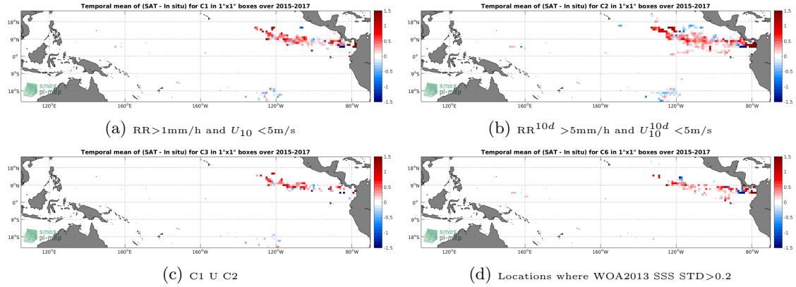
Figure 11: Temporal mean gridded over spatial boxes of size 1^\circ \times 1^\circ of \Delta SSS (SMAP-L3-JPL-V4-8DAY-RUNNING-60KM - Surface drifters) for 4 different subdatasets corresponding to: RR > 1\text{mm/h} and U_{10} < 5\text{m/s} (a), RR^{10d} > 5\text{mm/h} and U_{10}^{10d} < 5\text{m/s} (b), C1 U C2 (c), Locations where WOA2013 SSS STD > 0.2 (d).
