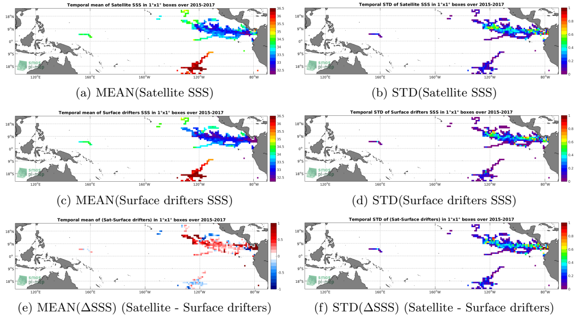
Figure 5: Temporal mean (left) and STD (right) of SSS from SMAP-L3-JPL-V4-8DAY-RUNNING-60KM (top), Surface drifters (middle), and of \Delta SSS (Satellite - Surface drifters). Only match-up pairs are used to generate these maps.
