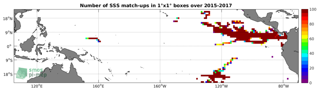
Figure 3: Number of SSS match-ups between Surface drifters SSS and the SMAP-L3-JPL-V4-8DAY-RUNNING-60KM SSS product for the Tropical Pacific Ocean Pi-MEP region over 1^\circ \times 1^\circ boxes and for the full satellite product period.
