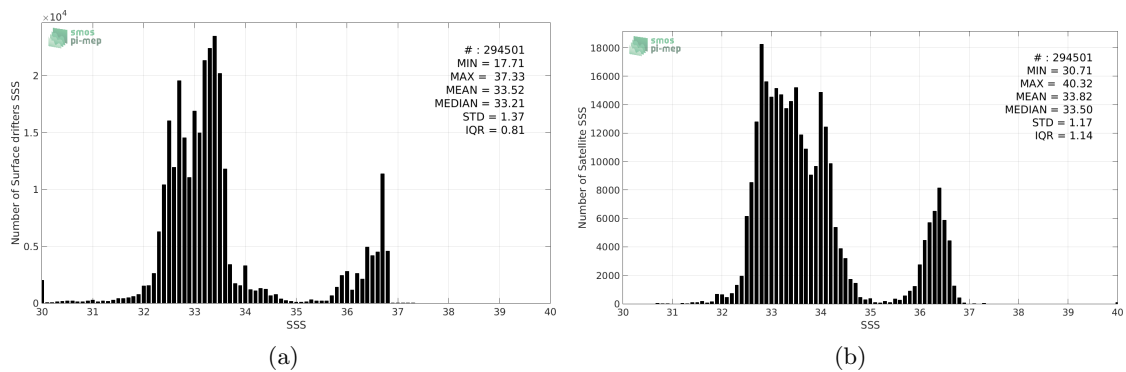
Figure 2: Histograms of SSS from Surface drifters (a) and SMAP-L3-JPL-V4-8DAY-RUNNING-60KM (b) considering all match-up pairs per bins of 0.1 over the Tropical Pacific Ocean Pi-MEP region and for the full satellite product period.
