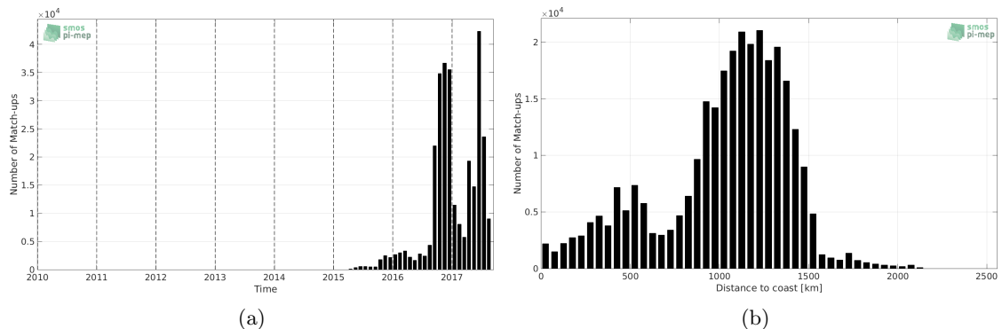
Figure 1: Number of match-ups between Surface drifters and SMAP-L3-JPL-V4-8DAY-RUNNING-60KM SSS as a function of time (a) and as function of the distance to coast (b) over the Tropical Pacific Ocean Pi-MEP region and for the full satellite product period.
