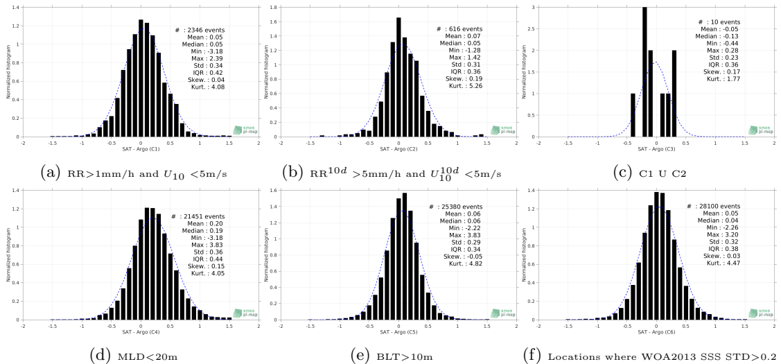
Figure 13: Normalized histogram of \Delta SSS (SMAP-L3-JPL-V4-8DAY-RUNNING-60KM - Argo) for 6 different subdatasets corresponding to: RR>1mm/h and U_{10} < 5m/s (a), RR^{10d} > 5mm/h and U_{10}^{10d} < 5m/s (b), C1 U C2 (c),MLD<20m (d),BLT>10m (e),Locations where WOA2013 SSS STD>0.2 (f).
