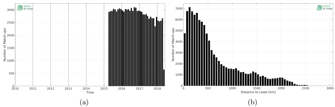
Figure 1: Number of match-ups between Argo and SMAP-L3-JPL-V4-8DAY-RUNNING-60KM SSS as a function of time (a) and as function of the distance to coast (b) over the Tropical Pacific Ocean Pi-MEP region and for the full satellite product period.
