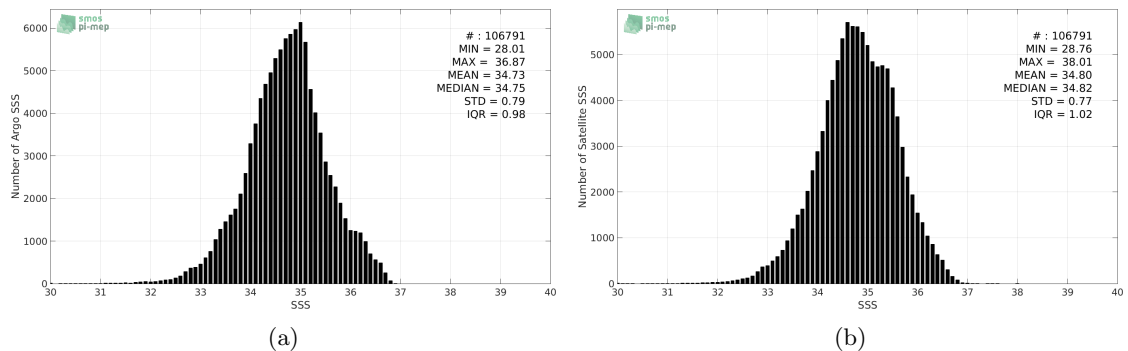
Figure 2: Histograms of SSS from Argo (a) and SMAP-L3-JPL-V4-8DAY-RUNNING-60KM (b) considering all match-up pairs per bins of 0.1 over the Tropical Pacific Ocean Pi-MEP region and for the full satellite product period.
