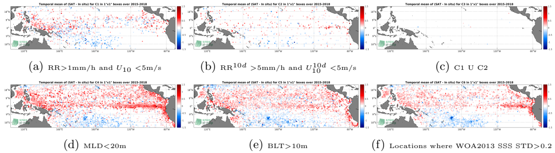
Figure 12: Temporal mean gridded over spatial boxes of size 1°x1° of \Delta SSS (SMAP-L3-JPL-V4-8DAY-RUNNING-60KM - Argo) for 6 different subdatasets corresponding to:RR>1mm/h and U_{10} < 5m/s (a), RR^{10d} > 5mm/h and U_{10}^{10d} < 5m/s (b), C1 U C2 (c),MLD<20m (d),BLT>10m (e),Locations where WOA2013 SSS STD>0.2 (f).
