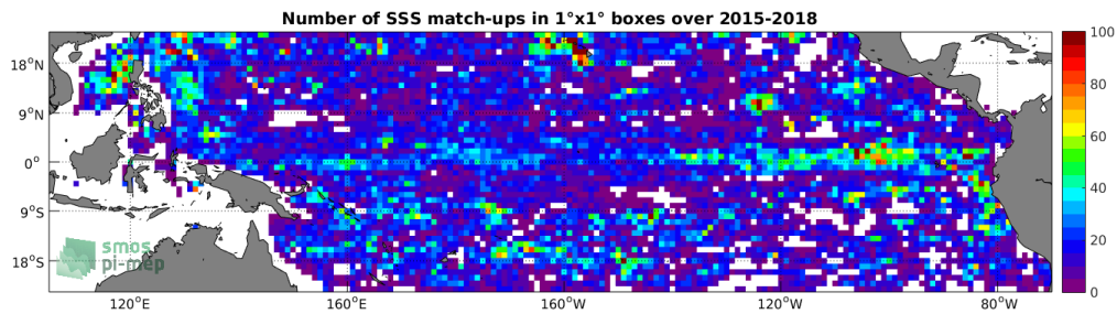
Figure 4: Number of SSS match-ups between Argo SSS and the SMAP-L3-JPL-V4-8DAY-RUNNING-60KM SSS product for the Tropical Pacific Ocean Pi-MEP region over 1^\circ \times 1^\circ boxes and for the full satellite product period.
