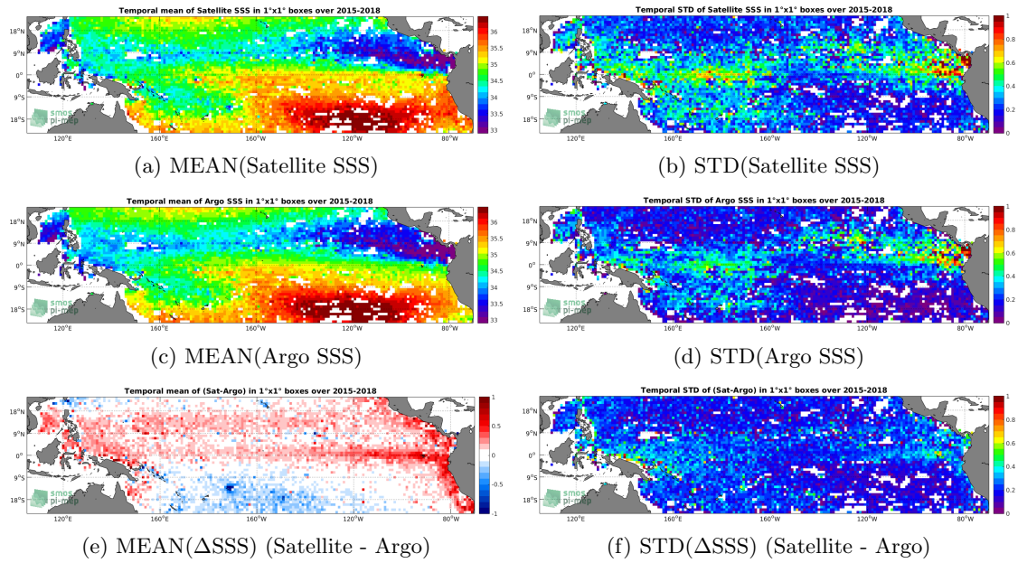
Figure 6: Temporal mean (left) and STD (right) of SSS from SMAP-L3-JPL-V4-8DAY-RUNNING-60KM (top), Argo (middle), and of \Delta SSS (Satellite - Argo). Only match-up pairs are used to generate these maps.
