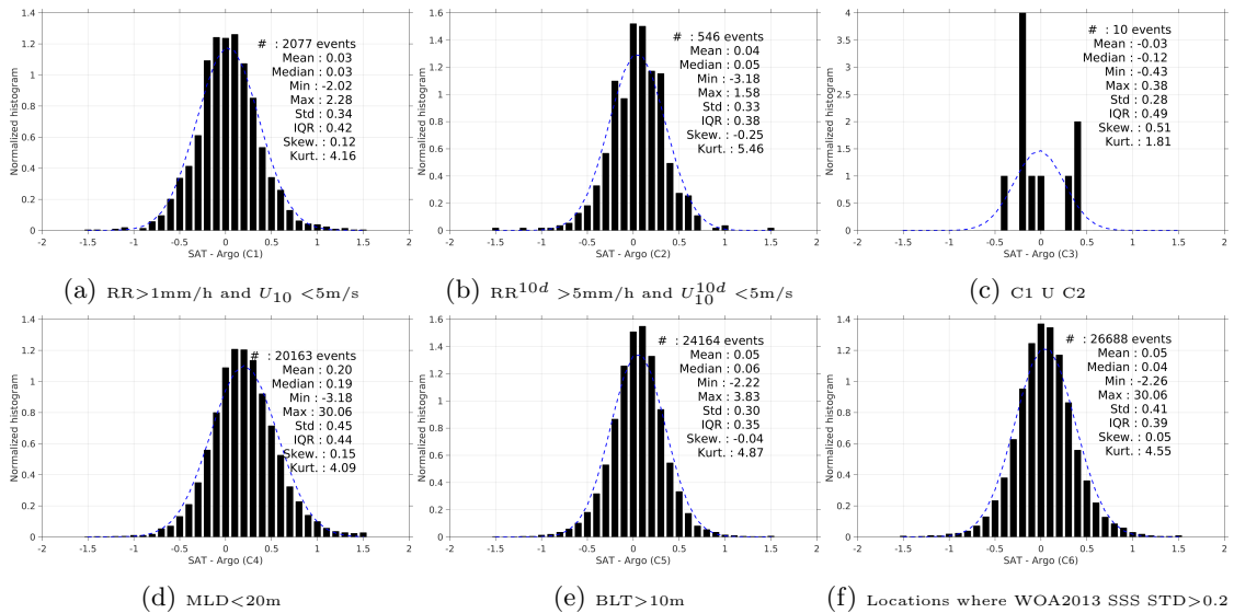
Figure 13: Normalized histogram of \Delta SSS (SMAP-L3-JPL-V4-8DAY-RUNNING-60KM - Argo) for 6 different subdatasets corresponding to: RR>1mm/h and U_{10} < 5 m/s (a), RR^{10d} > 5 mm/h and U_{10}^{10d} < 5 m/s (b), C1 U C2 (c),MLD<20m (d),BLT>10m (e),Locations where WOA2013 SSS STD>0.2 (f).
