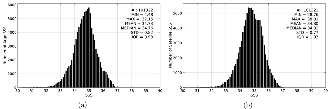
Figure 2: Histograms of SSS from Argo (a) and SMAP-L3-JPL-V4-8DAY-RUNNING-60KM (b) considering all match-up pairs per bins of 0.1 over the Tropical Pacific Ocean Pi-MEP region and for the full satellite product period.
