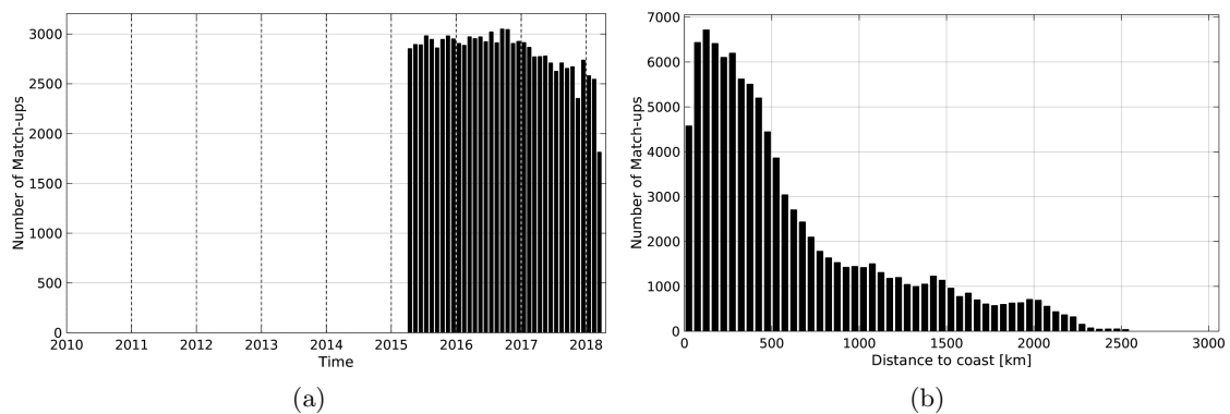
Figure 1: Number of match-ups between Argo and SMAP-L3-JPL-V4-8DAY-RUNNING-60KM SSS as a function of time (a) and as function of the distance to coast (b) over the Tropical Pacific Ocean Pi-MEP region and for the full satellite product period.
