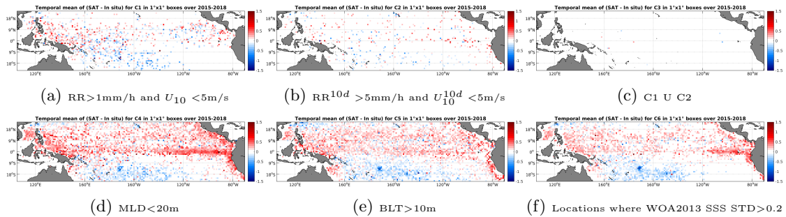
Figure 12: Temporal mean gridded over spatial boxes of size 1°x1° of \Delta SSS (SMAP-L3-JPL-V4-8DAY-RUNNING-60KM - Argo) for 6 different subdatasets corresponding to:RR>1mm/h and U_{10} < 5 m/s (a), RR^{10d} > 5 mm/h and U_{10}^{10d} < 5 m/s (b), C1 U C2 (c),MLD<20m (d),BLT>10m (e),Locations where WOA2013 SSS STD>0.2 (f).
