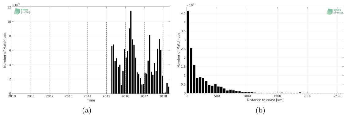
Figure 1: Number of match-ups between TSG-SAMOS and SMAP-L3-JPL-V4-MONTHLY-60KM SSS as a function of time (a) and as function of the distance to coast (b) over the Tropical Pacific Ocean Pi-MEP region and for the full satellite product period.
