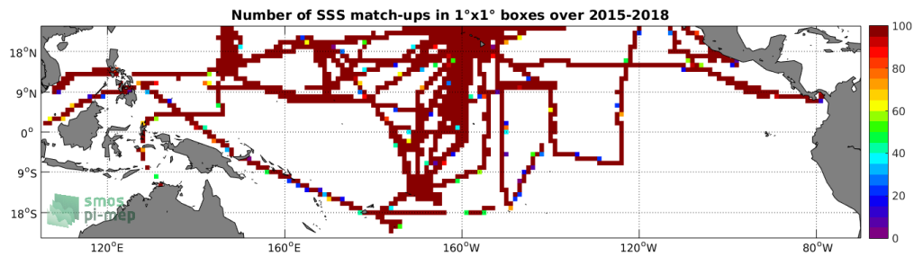
Figure 4: Number of SSS match-ups between TSG-SAMOS SSS and the SMAP-L3-JPL-V4-MONTHLY-60KM SSS product for the Tropical Pacific Ocean Pi-MEP region over 1^\circ \times 1^\circ boxes and for the full satellite product period.
