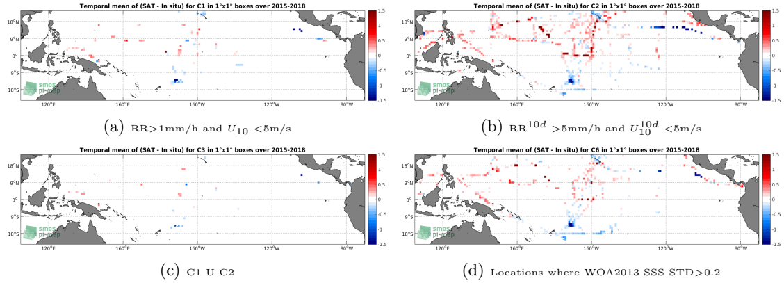
Figure 12: Temporal mean gridded over spatial boxes of size 1^\circ \times 1^\circ of \Delta SSS (SMAP-L3-JPL-V4-MONTHLY-60KM - TSG-SAMOS) for 4 different subdatasets corresponding to: RR > 1mm/h and U_{10} < 5\text{m/s} (a), RR 10d > 5mm/h and U_{10}^{10d} < 5\text{m/s} (b), C1 U C2 (c), Locations where WOA2013 SSS STD > 0.2 (d).
