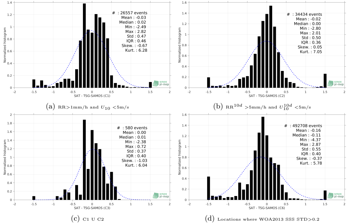
Figure 13: Normalized histogram of \Delta SSS (SMAP-L3-JPL-V4-MONTHLY-60KM - TSG-SAMOS) for 6 different subdatasets corresponding to: RR > 1\text{mm/h} and U_{10} < 5\text{m/s} (a), RR^{10d} > 5\text{mm/h} and U_{10}^{10d} < 5\text{m/s} (b), C1 U C2 (c), Locations where WOA2013 SSS STD > 0.2 (d).
