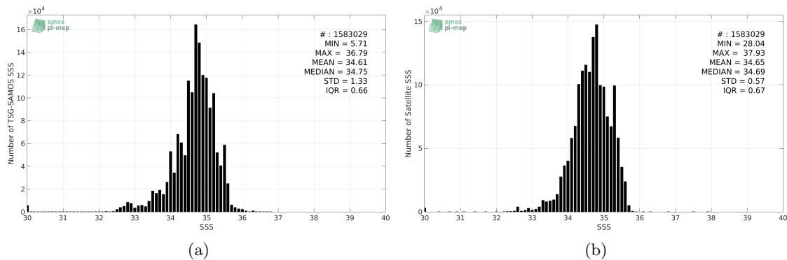
Figure 2: Histograms of SSS from TSG-SAMOS (a) and SMAP-L3-JPL-V4-MONTHLY-60KM (b) considering all match-up pairs per bins of 0.1 over the Tropical Pacific Ocean Pi-MEP region and for the full satellite product period.
