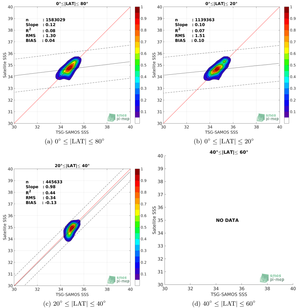
Figure 9: Contour maps of the concentration of SMAP-L3-JPL-V4-MONTHLY-60KM SSS (y-axis) versus TSG-SAMOS SSS (x-axis) at match-up pairs for different latitude bands. For each plot, the red line shows x=y . The black thin and dashed lines indicate a linear fit through the data cloud and the \pm 95\% confidence levels, respectively. The number match-up pairs n , the slope and R^2 coefficient of the linear fit, the root mean square (RMS) and the mean bias between satellite and in situ data are indicated for each latitude band in each plots.
