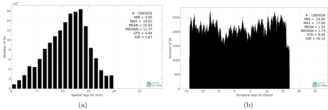
Figure 5: Histograms of the spatial (a) and temporal (b) lags between the time of the TSG-SAMOS measurements and the date of the corresponding SMAP-L3-JPL-V4-MONTHLY-60KM SSS product.
