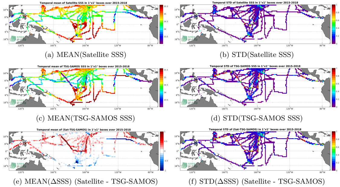
Figure 6: Temporal mean (left) and STD (right) of SSS from SMAP-L3-JPL-V4-MONTHLY-60KM (top), TSG-SAMOS (middle), and of \Delta SSS (Satellite - TSG-SAMOS). Only match-up pairs are used to generate these maps.
