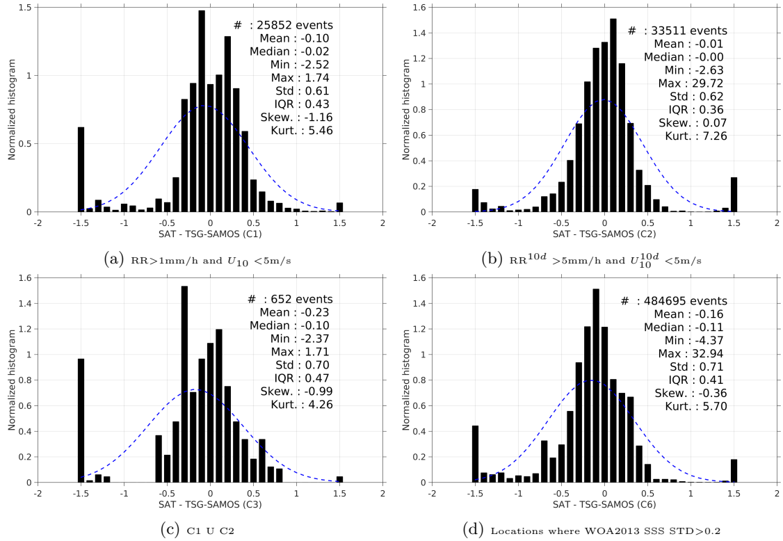
Figure 13: Normalized histogram of \Delta SSS (SMAP-L3-JPL-V4-MONTHLY-60KM - TSG-SAMOS) for 6 different subdatasets corresponding to: RR > 1mm/h and U_{10} < 5 m/s (a), RR^{10d} > 5 mm/h and U_{10}^{10d} < 5 m/s (b), C1 U C2 (c), Locations where WOA2013 SSS STD > 0.2 (d).
