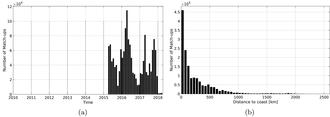
Figure 1: Number of match-ups between TSG-SAMOS and SMAP-L3-JPL-V4-MONTHLY-60KM SSS as a function of time (a) and as function of the distance to coast (b) over the Tropical Pacific Ocean Pi-MEP region and for the full satellite product period.
