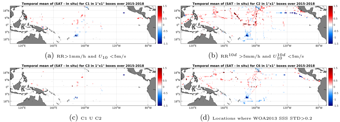
Figure 12: Temporal mean gridded over spatial boxes of size 1^\circ \times 1^\circ of \Delta SSS (SMAP-L3-JPL-V4-MONTHLY-60KM - TSG-SAMOS) for 4 different subdatasets corresponding to: RR > 1\text{mm/h} and U_{10} < 5\text{m/s} (a), RR^{10d} > 5\text{mm/h} and U_{10}^{10d} < 5\text{m/s} (b), C1 U C2 (c), Locations where WOA2013 SSS STD > 0.2 (d).
