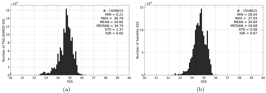
Figure 2: Histograms of SSS from TSG-SAMOS (a) and SMAP-L3-JPL-V4-MONTHLY-60KM (b) considering all match-up pairs per bins of 0.1 over the Tropical Pacific Ocean Pi-MEP region and for the full satellite product period.
