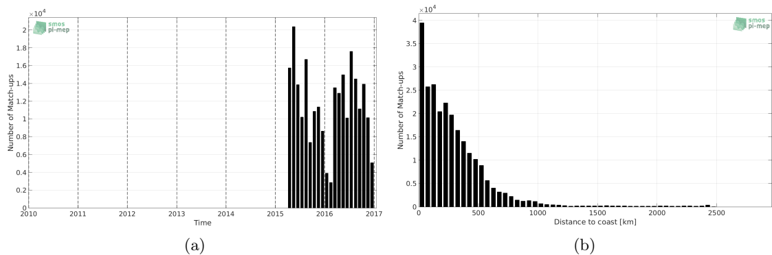
Figure 1: Number of match-ups between TSG-LEGOS-DM and SMAP-L3-JPL-V4-MONTHLY-60KM SSS as a function of time (a) and as function of the distance to coast (b) over the Tropical Pacific Ocean Pi-MEP region and for the full satellite product period.
