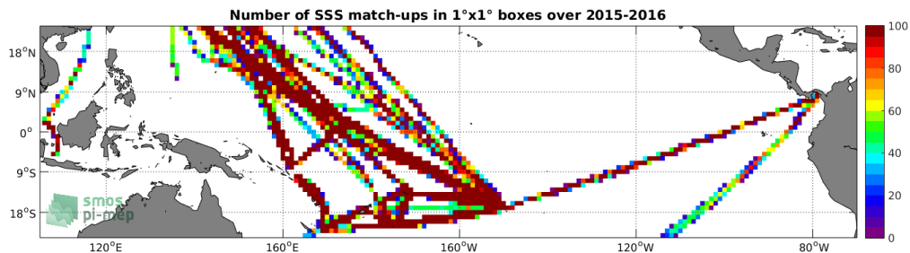
Figure 4: Number of SSS match-ups between TSG-LEGOS-DM SSS and the SMAP-L3-JPL-V4-MONTHLY-60KM SSS product for the Tropical Pacific Ocean Pi-MEP region over 1^\circ \times 1^\circ boxes and for the full satellite product period.
