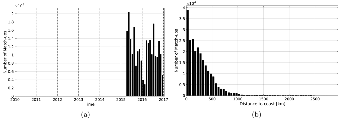
Figure 1: Number of match-ups between TSG-LEGOS-DM and SMAP-L3-JPL-V4-MONTHLY-60KM SSS as a function of time (a) and as function of the distance to coast (b) over the Tropical Pacific Ocean Pi-MEP region and for the full satellite product period.
