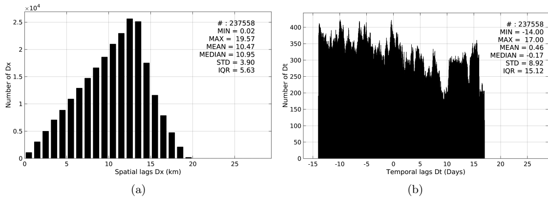
Figure 5: Histograms of the spatial (a) and temporal (b) lags between the time of the TSG-LEGOS-DM measurements and the date of the corresponding SMAP-L3-JPL-V4-MONTHLY-60KM SSS product.
