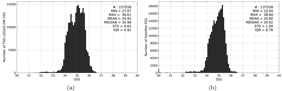
Figure 2: Histograms of SSS from TSG-LEGOS-DM (a) and SMAP-L3-JPL-V4-MONTHLY-60KM (b) considering all match-up pairs per bins of 0.1 over the Tropical Pacific Ocean Pi-MEP region and for the full satellite product period.
