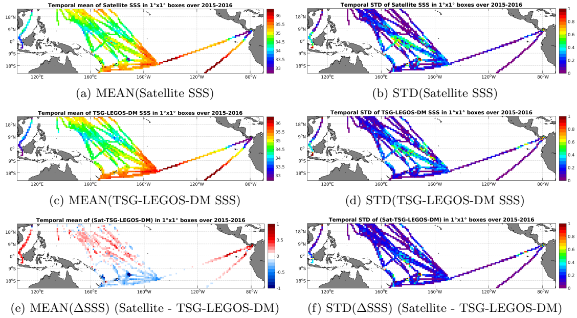
Figure 6: Temporal mean (left) and STD (right) of SSS from SMAP-L3-JPL-V4-MONTHLY-60KM (top), TSG-LEGOS-DM (middle), and of \Delta SSS (Satellite - TSG-LEGOS-DM). Only match-up pairs are used to generate these maps.
