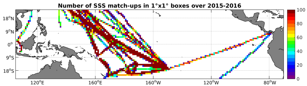
Figure 4: Number of SSS match-ups between TSG-LEGOS-DM SSS and the SMAP-L3-JPL-V4-MONTHLY-60KM SSS product for the Tropical Pacific Ocean Pi-MEP region over 1^\circ \times 1^\circ boxes and for the full satellite product period.
