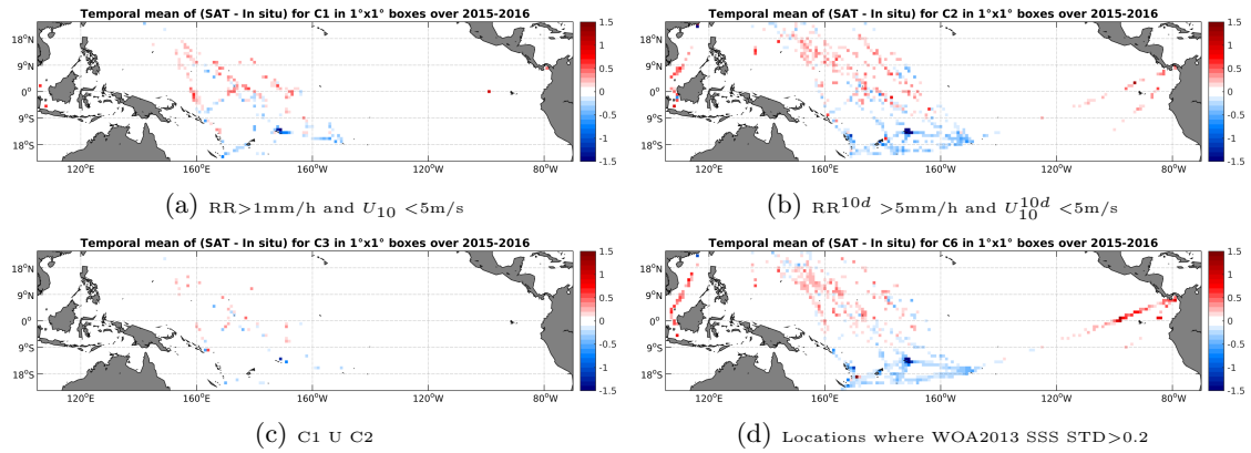
Figure 12: Temporal mean gridded over spatial boxes of size 1^\circ \times 1^\circ of \Delta SSS (SMAP-L3-JPL-V4-MONTHLY-60KM - TSG-LEGOS-DM) for 4 different subdatasets corresponding to: RR > 1\text{mm/h} and U_{10} < 5\text{m/s} (a), RR^{10d} > 5\text{mm/h} and U_{10}^{10d} < 5\text{m/s} (b), C1 U C2 (c), Locations where WOA2013 SSS STD > 0.2 (d).
