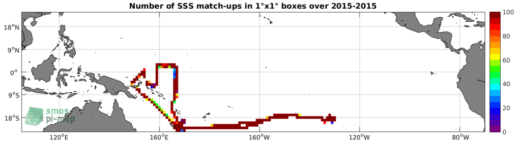
Figure 4: Number of SSS match-ups between TSG-GOSUD-Research-vessel SSS and the SMAP-L3-JPL-V4-MONTHLY-60KM SSS product for the Tropical Pacific Ocean Pi-MEP region over 1^\circ \times 1^\circ boxes and for the full satellite product period.
