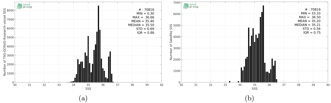
Figure 2: Histograms of SSS from TSG-GOSUD-Research-vessel (a) and SMAP-L3-JPL-V4-MONTHLY-60KM (b) considering all match-up pairs per bins of 0.1 over the Tropical Pacific Ocean Pi-MEP region and for the full satellite product period.
