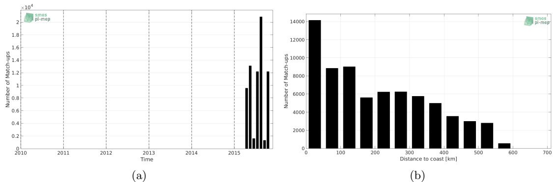
Figure 1: Number of match-ups between TSG-GOSUD-Research-vessel and SMAP-L3-JPL-V4-MONTHLY-60KM SSS as a function of time (a) and as function of the distance to coast (b) over the Tropical Pacific Ocean Pi-MEP region and for the full satellite product period.
