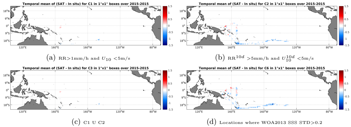
Figure 12: Temporal mean gridded over spatial boxes of size 1^\circ \times 1^\circ of \Delta SSS (SMAP-L3-JPL-V4-MONTHLY-60KM - TSG-GOSUD-Research-vessel) for 4 different subdatasets corresponding to: RR > 1\text{mm/h} and U_{10} < 5\text{m/s} (a), RR^{10d} > 5\text{mm/h} and U_{10}^{10d} < 5\text{m/s} (b), C1 U C2 (c), Locations where WOA2013 SSS STD > 0.2 (d).
