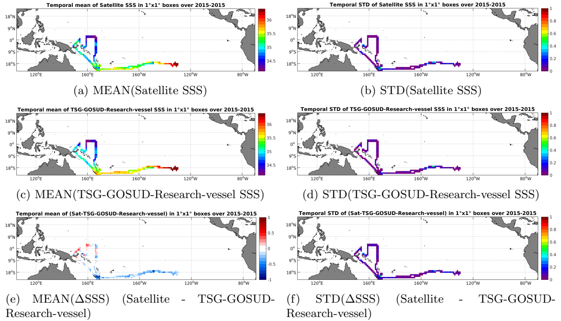
Figure 6: Temporal mean (left) and STD (right) of SSS from SMAP-L3-JPL-V4-MONTHLY-60KM (top), TSG-GOSUD-Research-vessel (middle), and of \Delta SSS (Satellite - TSG-GOSUD-Research-vessel). Only match-up pairs are used to generate these maps.
