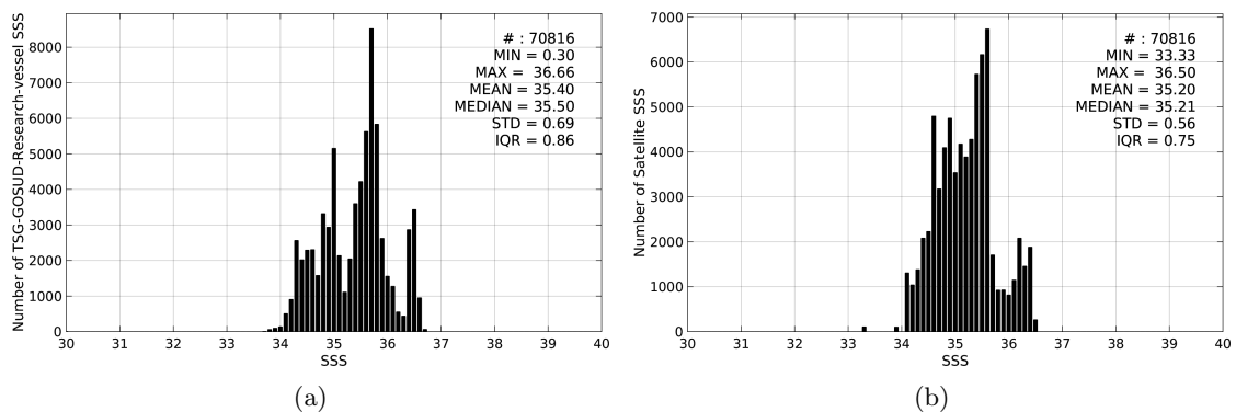
Figure 2: Histograms of SSS from TSG-GOSUD-Research-vessel (a) and SMAP-L3-JPL-V4-MONTHLY-60KM (b) considering all match-up pairs per bins of 0.1 over the Tropical Pacific Ocean Pi-MEP region and for the full satellite product period.
