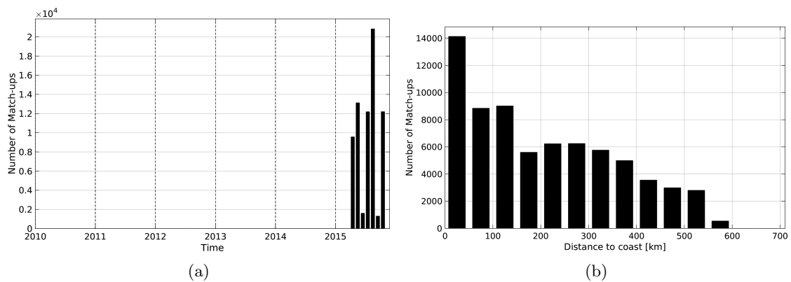
Figure 1: Number of match-ups between TSG-GOSUD-Research-vessel and SMAP-L3-JPL-V4-MONTHLY-60KM SSS as a function of time (a) and as function of the distance to coast (b) over the Tropical Pacific Ocean Pi-MEP region and for the full satellite product period.
