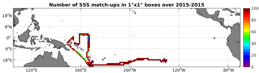
Figure 4: Number of SSS match-ups between TSG-GOSUD-Research-vessel SSS and the SMAP-L3-JPL-V4-MONTHLY-60KM SSS product for the Tropical Pacific Ocean Pi-MEP region over 1^\circ \times 1^\circ boxes and for the full satellite product period.
