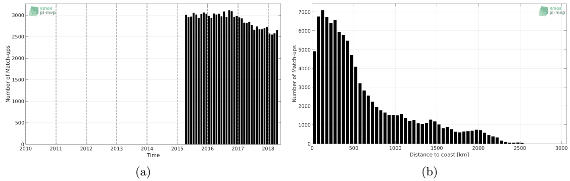
Figure 1: Number of match-ups between Argo and SMAP-L3-JPL-V4-MONTHLY-60KM SSS as a function of time (a) and as function of the distance to coast (b) over the Tropical Pacific Ocean Pi-MEP region and for the full satellite product period.
