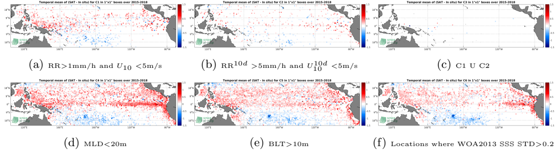
Figure 12: Temporal mean gridded over spatial boxes of size 1^\circ \times 1^\circ of \Delta\text{SSS} (SMAP-L3-JPL-V4-MONTHLY-60KM - Argo) for 6 different subdatasets corresponding to: \text{RR} > 1\text{mm/h} and U_{10} < 5\text{m/s} (a), \text{RR}^{10d} > 5\text{mm/h} and U_{10}^{10d} < 5\text{m/s} (b), C1 U C2 (c), \text{MLD} < 20\text{m} (d), \text{BLT} > 10\text{m} (e), Locations where WOA2013 SSS STD > 0.2 (f).
