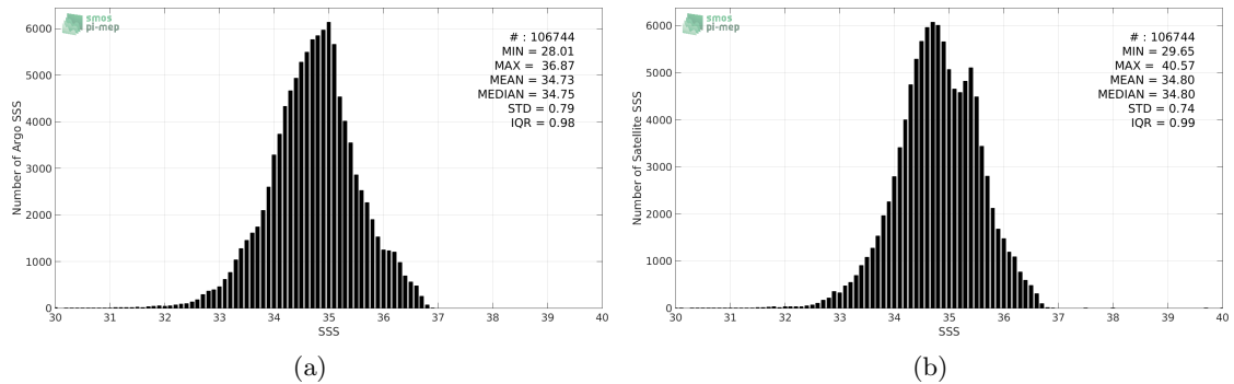
Figure 2: Histograms of SSS from Argo (a) and SMAP-L3-JPL-V4-MONTHLY-60KM (b) considering all match-up pairs per bins of 0.1 over the Tropical Pacific Ocean Pi-MEP region and for the full satellite product period.
