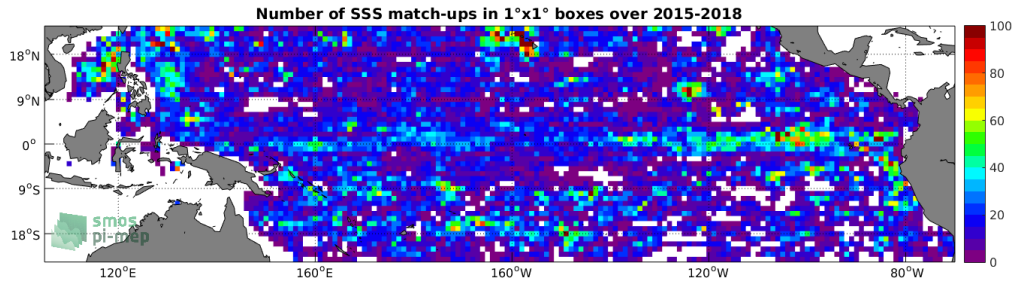
Figure 4: Number of SSS match-ups between Argo SSS and the SMAP-L3-JPL-V4-MONTHLY-60KM SSS product for the Tropical Pacific Ocean Pi-MEP region over 1^\circ \times 1^\circ boxes and for the full satellite product period.
