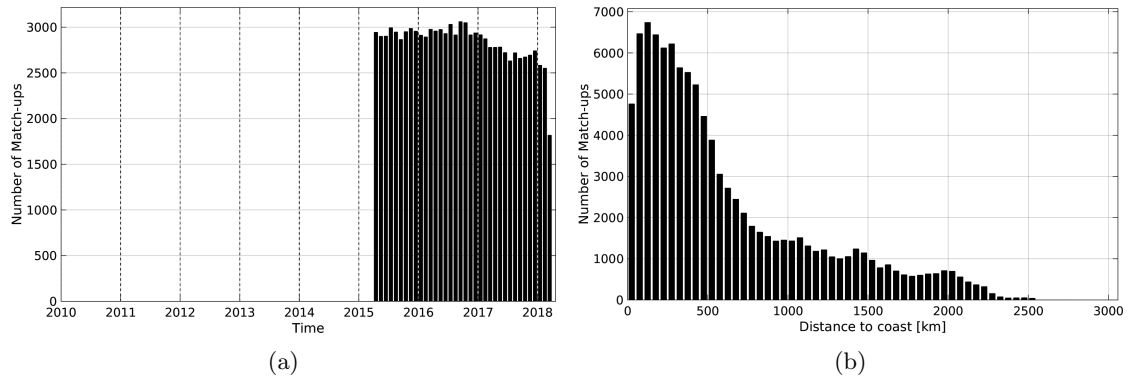
Figure 1: Number of match-ups between Argo and SMAP-L3-JPL-V4-MONTHLY-60KM SSS as a function of time (a) and as function of the distance to coast (b) over the Tropical Pacific Ocean Pi-MEP region and for the full satellite product period.
