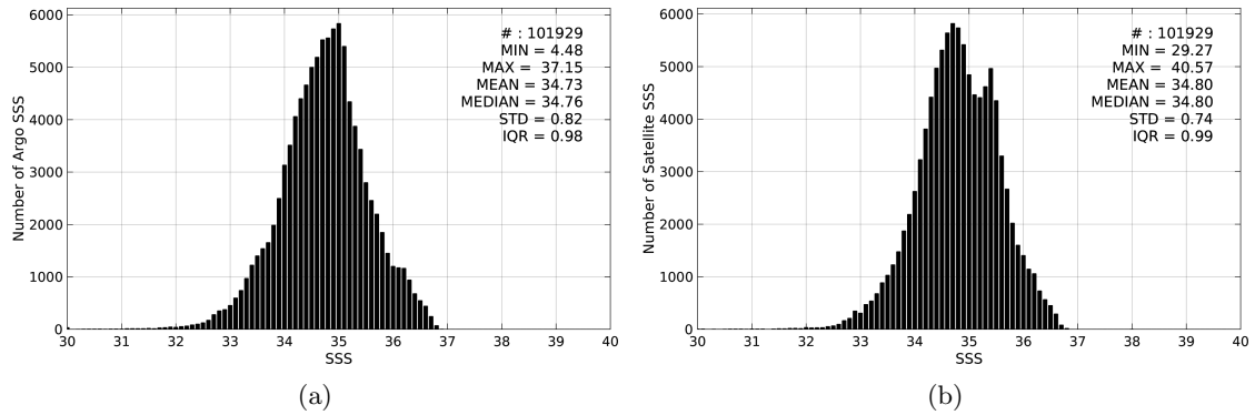
Figure 2: Histograms of SSS from Argo (a) and SMAP-L3-JPL-V4-MONTHLY-60KM (b) considering all match-up pairs per bins of 0.1 over the Tropical Pacific Ocean Pi-MEP region and for the full satellite product period.
