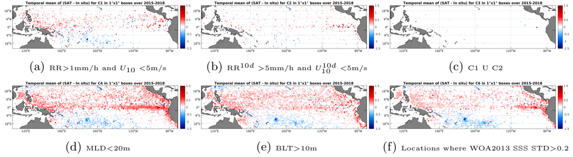
Figure 12: Temporal mean gridded over spatial boxes of size 1^\circ \times 1^\circ of \Delta SSS (SMAP-L3-JPL-V4-MONTHLY-60KM - Argo) for 6 different subdatasets corresponding to: RR > 1\text{mm/h} and U_{10} < 5\text{m/s} (a), RR^{10d} > 5\text{mm/h} and U_{10}^{10d} < 5\text{m/s} (b), C1 U C2 (c), MLD < 20\text{m} (d), BLT > 10\text{m} (e), Locations where WOA2013 SSS STD > 0.2 (f).
