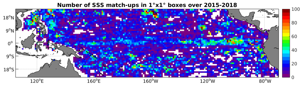
Figure 4: Number of SSS match-ups between Argo SSS and the SMAP-L3-JPL-V4-MONTHLY-60KM SSS product for the Tropical Pacific Ocean Pi-MEP region over 1°x1° boxes and for the full satellite product period.
