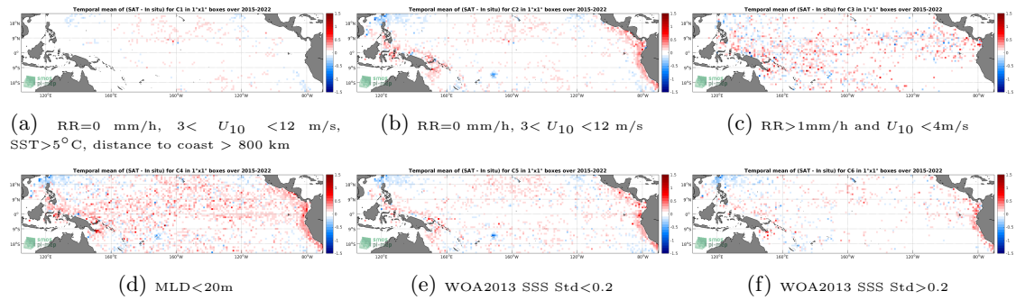
Figure 12: Temporal mean gridded over spatial boxes of size 1^\circ \times 1^\circ of \Delta SSS (SMAP SSS L2-AVERAGED v5 (RSS) - Argo) for 6 different subdatasets corresponding to:RR=0 mm/h, 3 < U_{10} < 12 m/s, SST >5^\circ C, distance to coast > 800 km (a), RR=0 mm/h, 3 < U_{10} < 12 m/s (b), RR >1 mm/h and U_{10} < 4 m/s (c),MLD <20 m (d),WOA2013 SSS Std <0.2 (e),WOA2013 SSS Std >0.2 (f).
