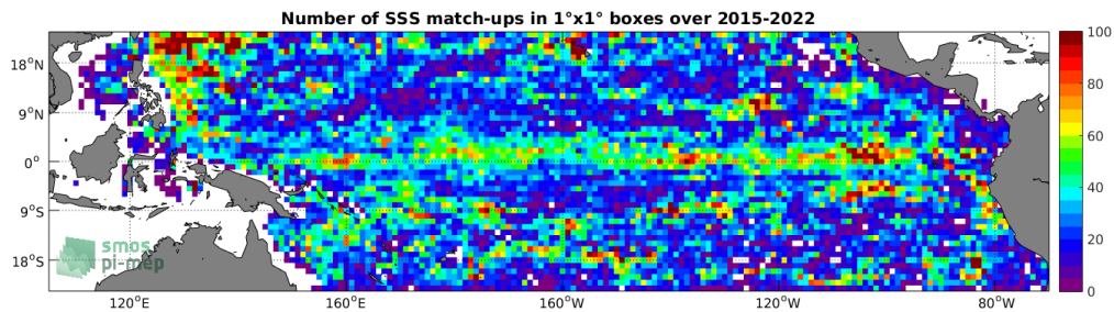
Figure 4: Number of SSS match-ups between Argo SSS and the SMAP SSS L2-AVERAGED v5 (RSS) SSS product for the Tropical Pacific Ocean Pi-MEP region over 1^\circ \times 1^\circ boxes and for the full satellite product period.
