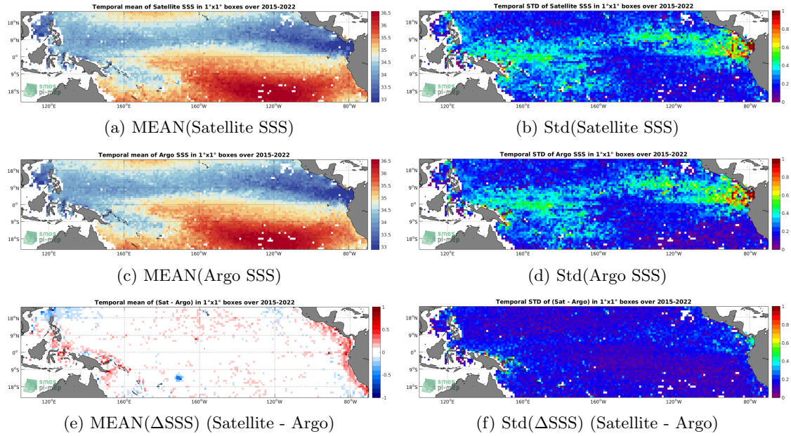
Figure 6: Temporal mean (left) and Std (right) of SSS from SMAP SSS L2-AVERAGED v5 (RSS) (top), Argo (middle), and of \Delta SSS (Satellite - Argo). Only match-up pairs are used to generate these maps.
