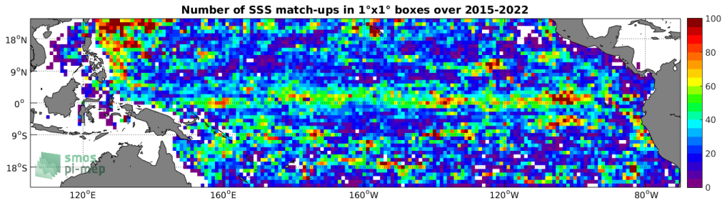
Figure 4: Number of SSS match-ups between Argo SSS and the SMAP SSS L2-AVERAGED v5.0 (JPL) SSS product for the Tropical Pacific Ocean Pi-MEP region over 1^\circ \times 1^\circ boxes and for the full satellite product period.
