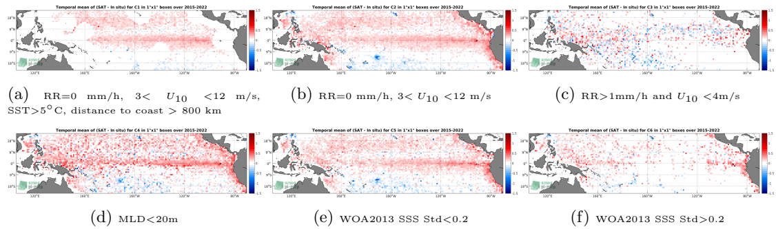
Figure 12: Temporal mean gridded over spatial boxes of size 1^\circ \times 1^\circ of \Delta SSS (SMAP SSS L2-AVERAGED v5.0 (JPL) - Argo) for 6 different subdatasets corresponding to:RR=0 mm/h, 3 < U_{10} < 12 m/s, SST >5^\circ C, distance to coast > 800 km (a), RR=0 mm/h, 3 < U_{10} < 12 m/s (b), RR >1 mm/h and U_{10} < 4 m/s (c),MLD <20 m (d),WOA2013 SSS Std <0.2 (e),WOA2013 SSS Std >0.2 (f).
