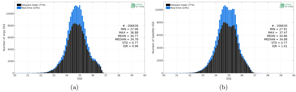
Figure 2: Histograms of SSS from Argo (a) and SMAP SSS L2-AVERAGED v5.0 (JPL) (b) considering all match-up pairs per bins of 0.1 over the Tropical Pacific Ocean Pi-MEP region and for the full satellite product period.
