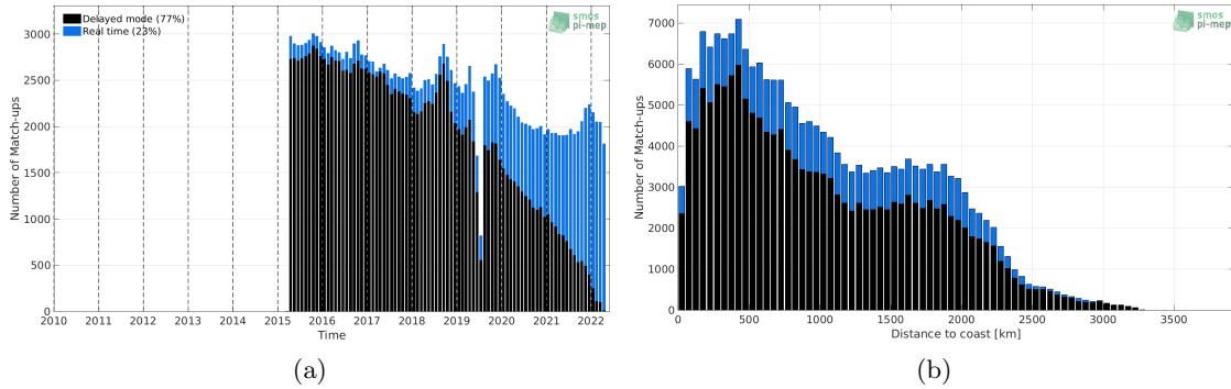
Figure 1: Number of match-ups between Argo and SMAP SSS L2-AVERAGED v5.0 (JPL) SSS as a function of time (a) and as function of the distance to coast (b) over the Tropical Pacific Ocean Pi-MEP region and for the full satellite product period.
