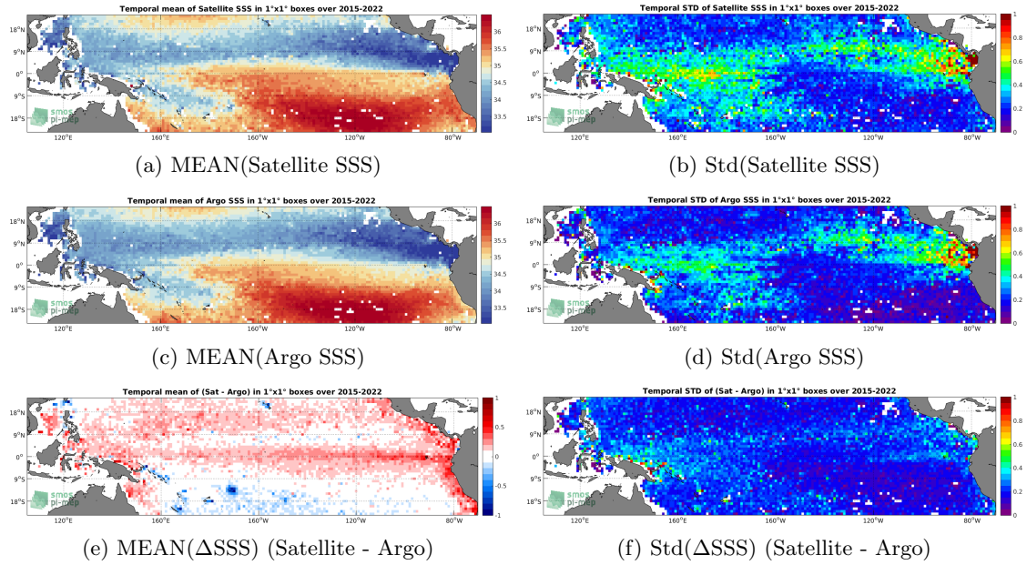
Figure 6: Temporal mean (left) and Std (right) of SSS from SMAP SSS L2-AVERAGED v5.0 (JPL) (top), Argo (middle), and of \Delta SSS (Satellite - Argo). Only match-up pairs are used to generate these maps.
